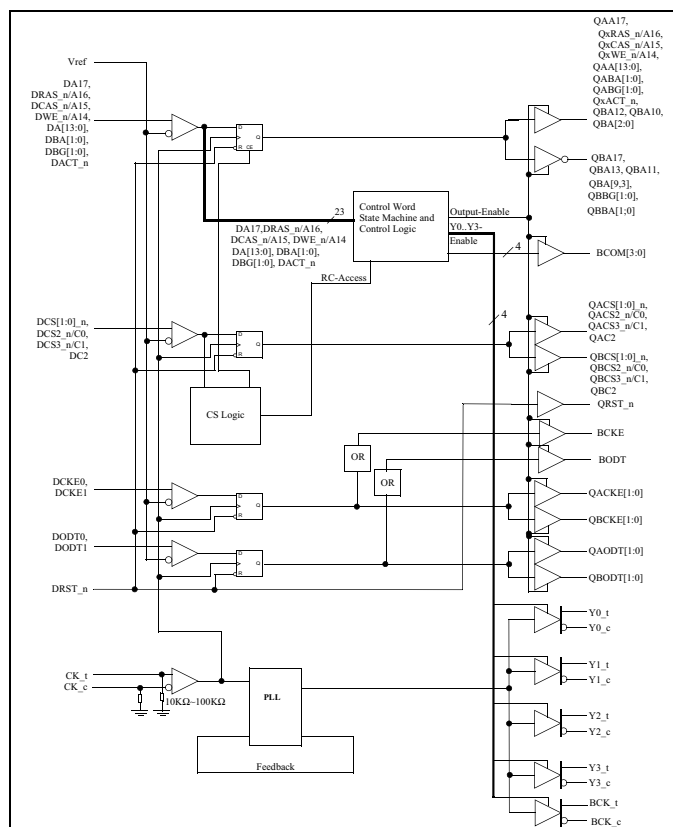
Figure 1. Block Diagram
