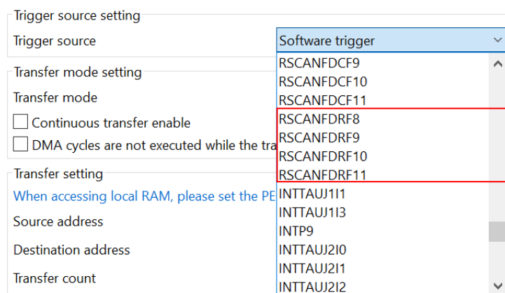
Figure 3-4 DMA Controller Trigger source setting
