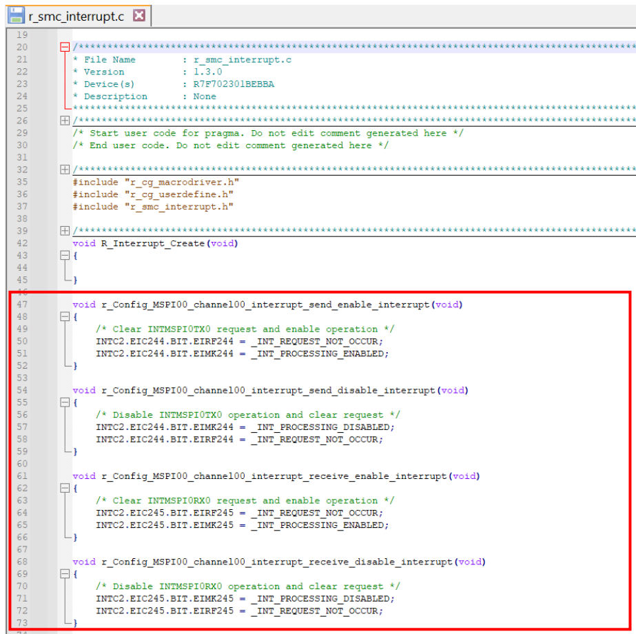
Figure 2-4 Interrupt Enable/Disable Functions Code Example
