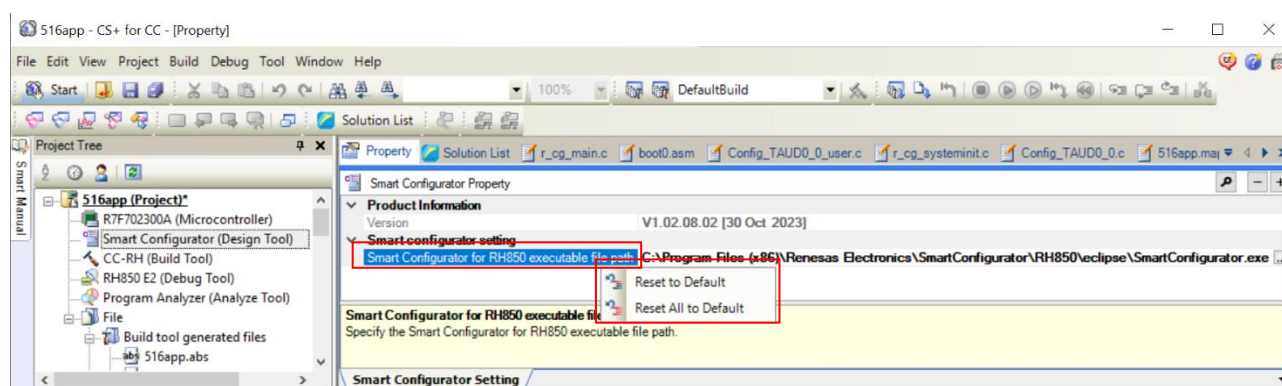
Figure 3-3 Change back to default installer path after clicking "Reset to Default" or "Reset All to Default"
