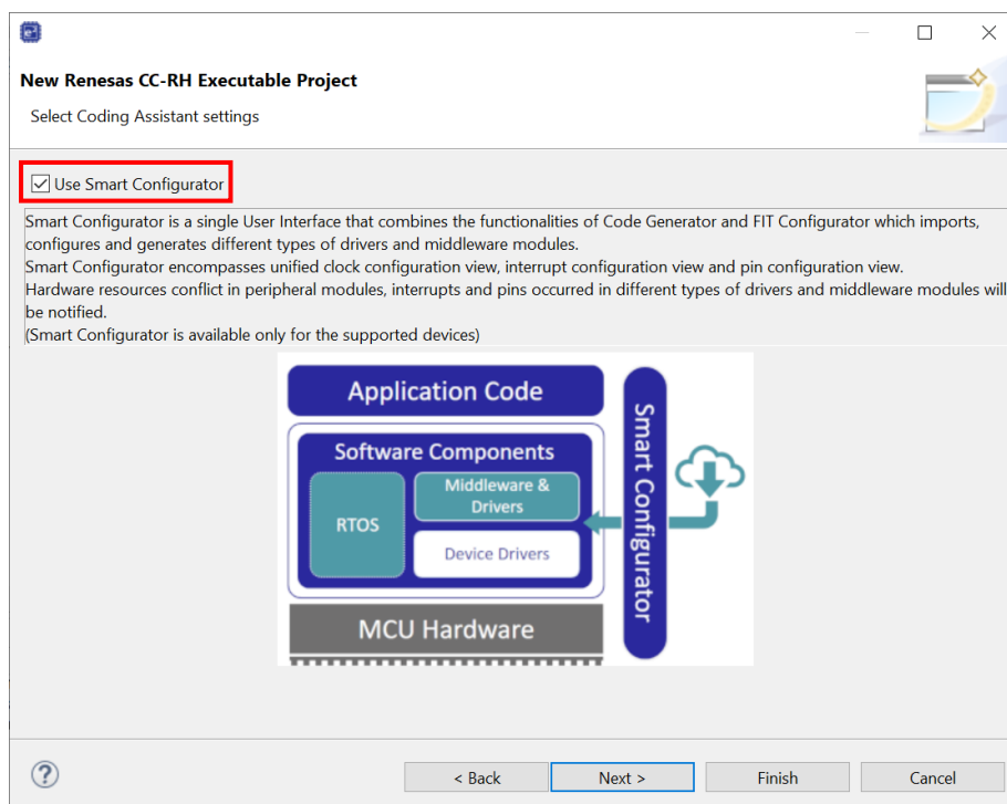
Figure 2-1 Support Smart Configurator for RH850 plug-in in e 2 studio
