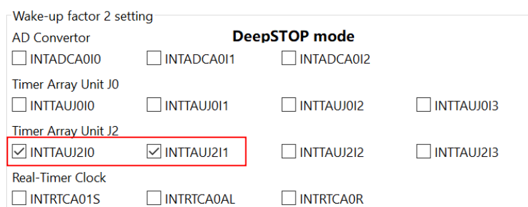
Figure 3-5 Wake-up factor 2 setting in DeepSTOP mode
