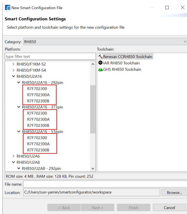
Figure 3-9 Device selection for RH850/U2A16
