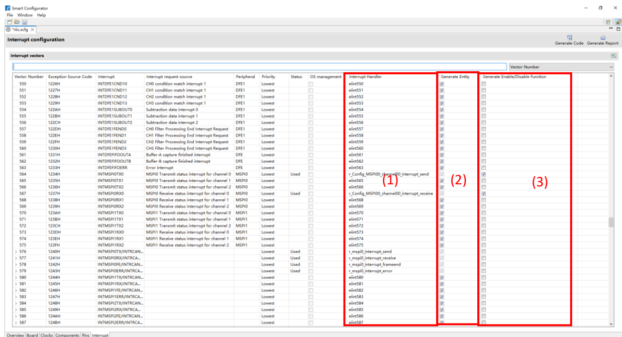
Figure 2-3 Interrupt Handler and Generate Entity settings
