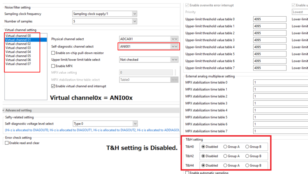
Figure 3-2. Virtual channel setting and T&H setting
