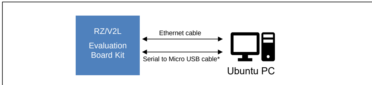
Figure 3-1 Hardware Configuration
