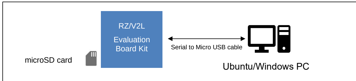
Figure 4-1 Hardware Configuration
