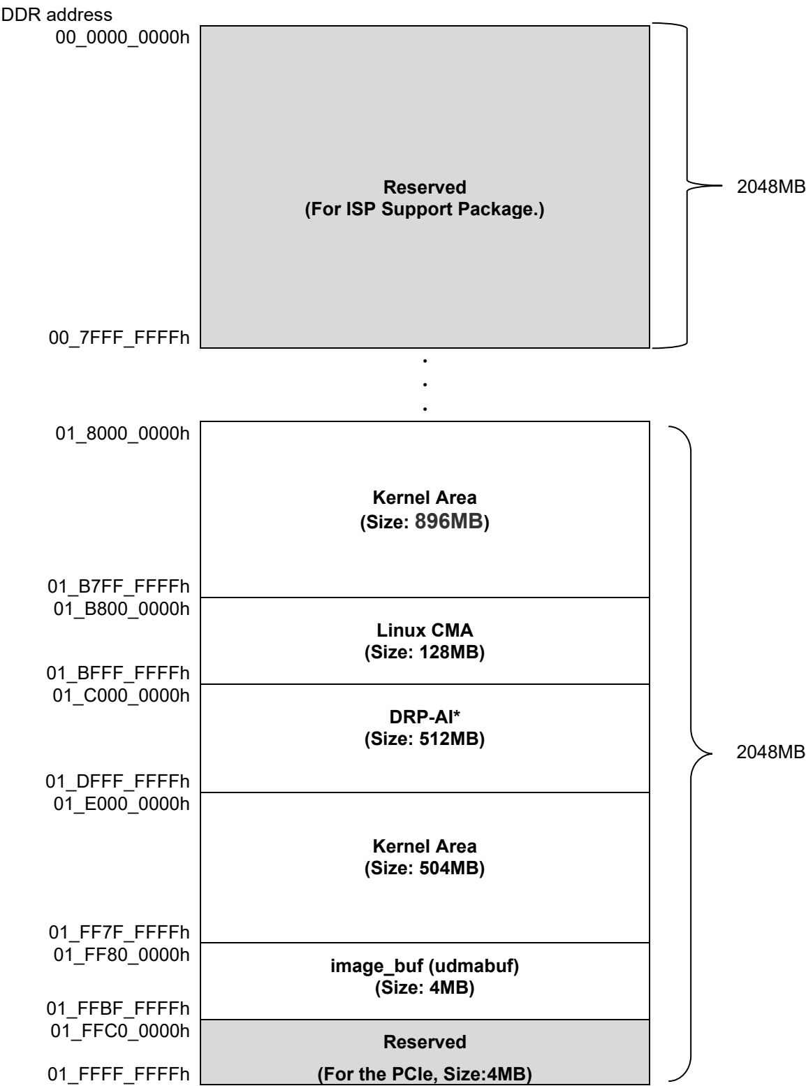
Figure 2. Memory Map
