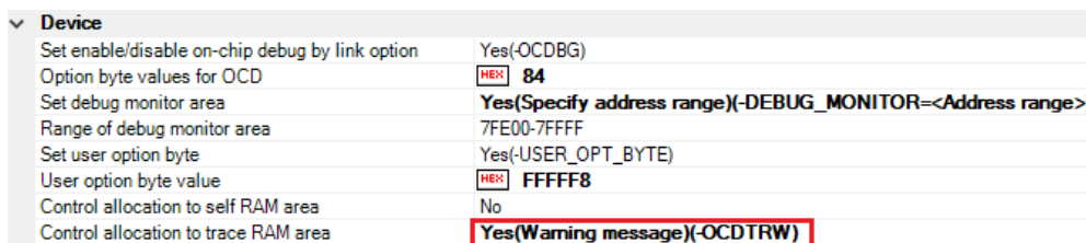
Figure 6-10 Select [Yes(Warning message)(-OCDTRW)] in CS+ [CCRL property]
