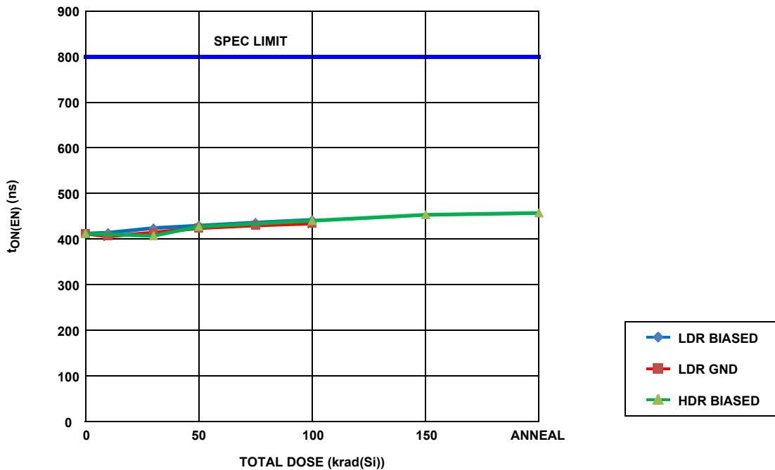
FIGURE 31. ISL7x840SEH enable to output ON delay, supply voltage \pm 15V , as a function of total dose irradiation at HDR for the biased (per Figure 2) case and at LDR for the unbiased (all pins grounded) and the biased (per Figure 2) cases. The LDR was 0.0089\text{rad(Si)}/\text{s} and the HDR was 69.72\text{rad(Si)}/\text{s} . Sample size for each of the three cells was 4. The post-irradiation SMD limit is 800ns maximum
