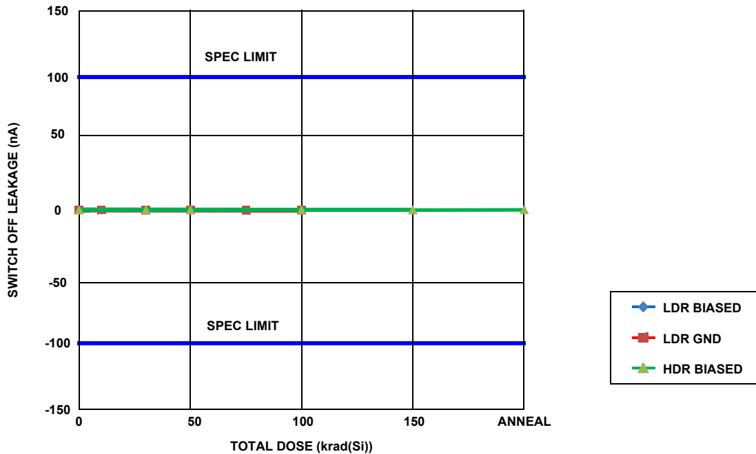
FIGURE 15. ISL7840SEH switch OFF leakage ( I_{S(OFF)} ) into the source of an unselected channel, average of all 16 channels, supply voltage \pm 15V , input voltage -11.5V as a function of total dose irradiation at HDR for the biased (per Figure 2) case and at LDR for the unbiased (all pins grounded) and the biased (per Figure 2) cases. The LDR was 0.0089\text{rad(Si)/s} and the HDR was 69.72\text{rad(Si)/s} . Sample size for each of the three cells was 4. The post-irradiation SMD limits are -100\text{nA} to 100\text{nA} .
