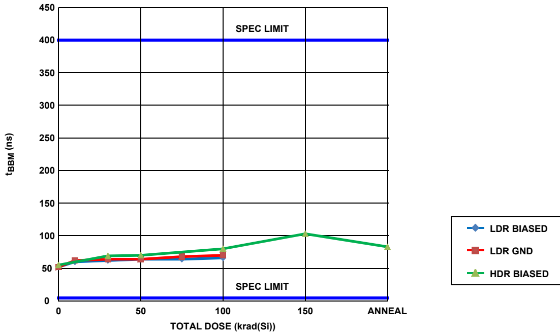
FIGURE 30. ISL7x840SEH break-before-make time delay, supply voltage \pm 15V , as a function of total dose irradiation at HDR for the biased (per Figure 2) case and at LDR for the unbiased (all pins grounded) and the biased (per Figure 2) cases. The LDR was 0.0089\text{rad(Si)}/\text{s} and the HDR was 69.72\text{rad(Si)}/\text{s} . Sample size for each of the three cells was 4. The post-irradiation SMD limits are 5ns to 400ns.
