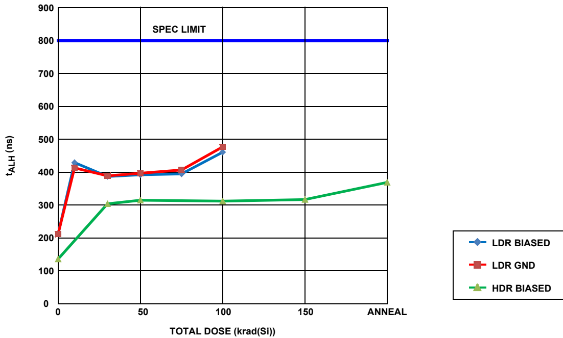
FIGURE 28. ISL7x840SEH address to output access time, LOW-to-HIGH, supply voltage ±15V, as a function of total dose irradiation at HDR for the biased case and at LDR for the unbiased (all pins grounded) and the biased (per Figure 2) cases. The LDR was 0.0089rad(Si)/s and the HDR was 69.72rad(Si)/s. Sample size for each of the three cells was 4. The post-irradiation SMD limit is 800ns maximum.
