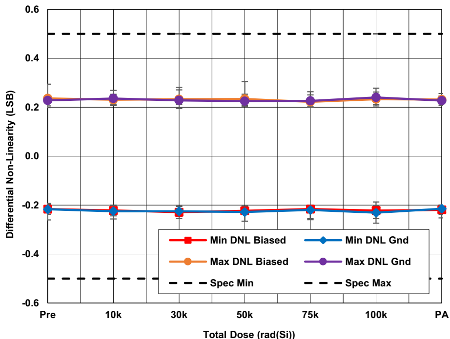
Figure 5. ISL73141SEHMFN average minimum and maximum differential non-linearity (DNL) with AV_{CC} = 3.3V , DV_{CC} = 2.5V , REF = 3.0V , f_{SAMP} = 750kps , and A_{IN} = full-scale sine wave as a function of LDR irradiation and anneal. The error bars represent the minimum and maximum measured values. The datasheet limits are -0.5 LSB minimum and 0.5 LSB maximum.
