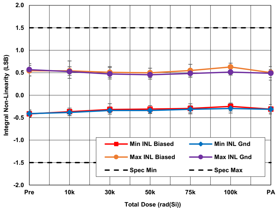
Figure 4. ISL73141SEHMFN average minimum and maximum integral non-linearity (INL) with AV_{CC} = 3.3V , DV_{CC} = 2.5V , REF = 3.0V , f_{SAMP} = 750kps , and A_{IN} = full-scale sine wave as a function of LDR irradiation and anneal. The error bars represent the minimum and maximum measured values. The datasheet limits are -1.5 LSB minimum and 1.5 LSB maximum.
