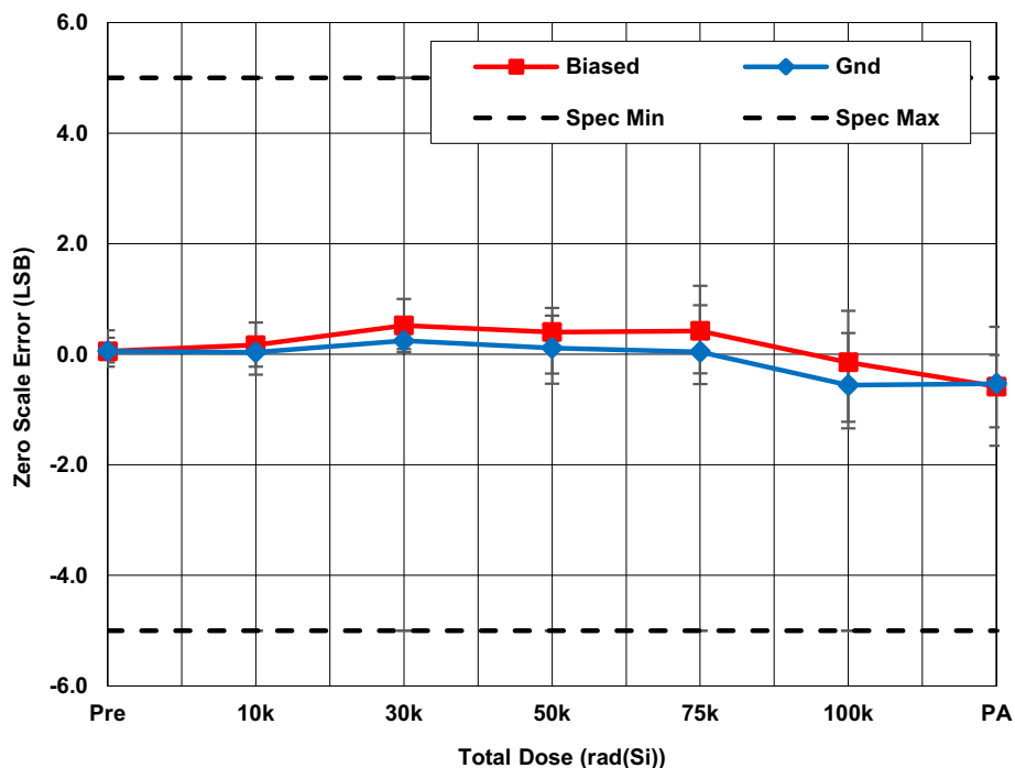
Figure 6. ISL73141SEHMFN average zero scale error (VOFF) with AV_{CC} = 3.3V , DV_{CC} = 2.5V , REF = 3.0V , f_{SAMP} = 750ksps , and A_{IN} = Gnd as a function of LDR irradiation and anneal. The error bars represent the minimum and maximum measured values. The datasheet limits are -5 LSB minimum and 5 LSB maximum.
