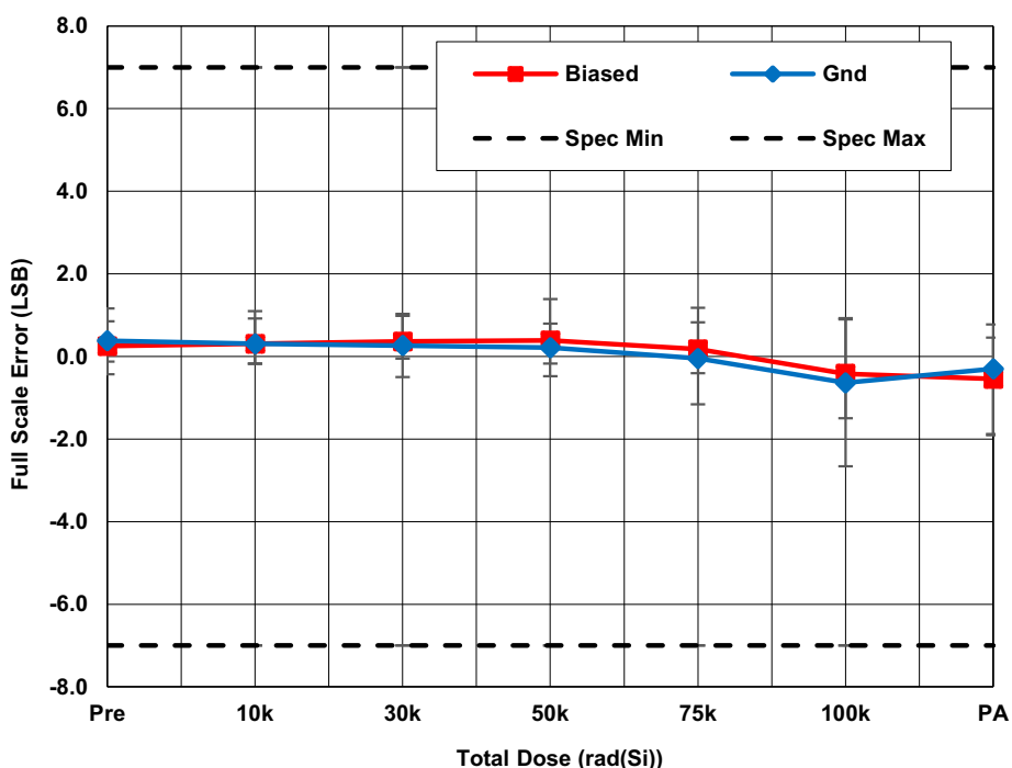
Figure 7. ISL73141SEHMFN average full-scale error (FSE) with AV_{CC} = 3.3V , DV_{CC} = 2.5V , REF = 3.0V , f_{SAMP} = 750ksps , and A_{IN} = VREF as a function of LDR irradiation and anneal. The error bars represent the minimum and maximum measured values. The datasheet limits are -7 LSB minimum and 7 LSB maximum.
