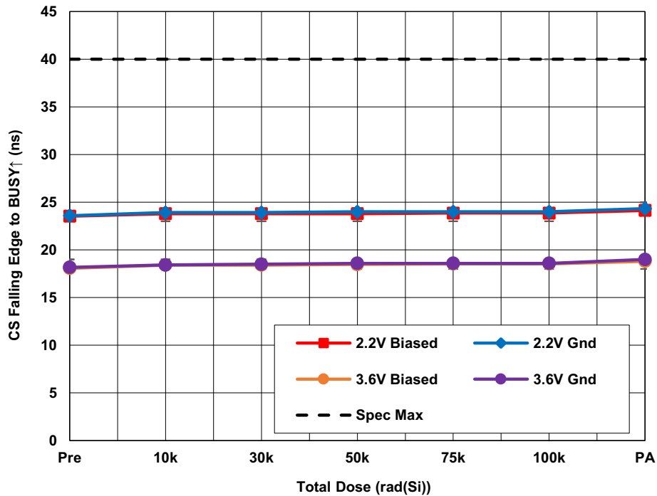
Figure 28. ISL73141SEHMFN average \overline{CS} falling edge to BUSY rising edge ( t_{BUSYLH} ) with AV_{CC} = 3.0V , DV_{CC} = 2.2V and AV_{CC} = 3.6V , DV_{CC} = 3.6V , REF = 3.0V , f_{SAMP} = 750ksps , A_{IN} = -1dbFS and C_L = 10pF as a function of LDR irradiation and anneal. The error bars represent the minimum and maximum measured values. The datasheet limit is 40ns maximum.
