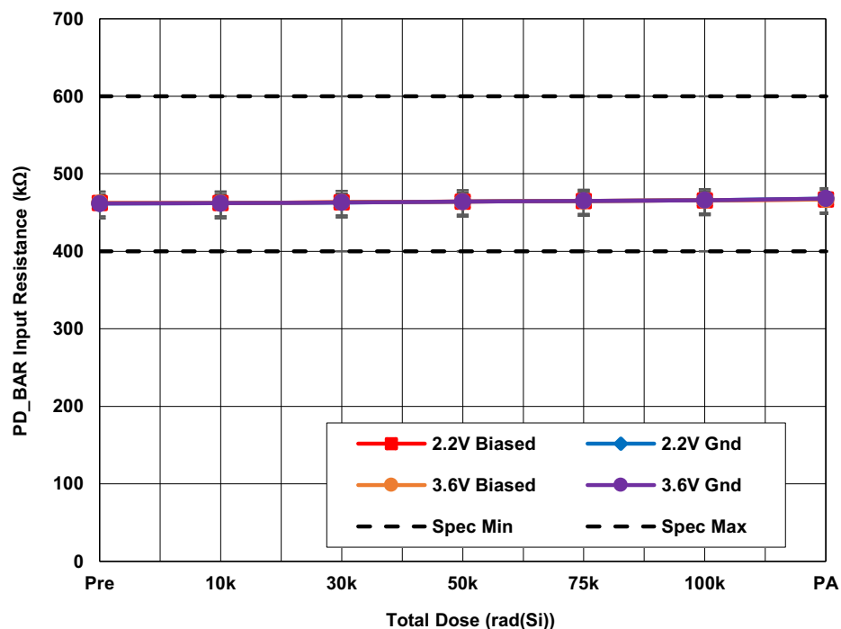
Figure 26. ISL73141SEHMFN average \overline{PD} input resistance ( R_{INPDL} ) with AV_{CC} = 3.3V , DV_{CC} = 3.6V and 2.2V and REF = 3.0V as a function of LDR irradiation and anneal. The error bars represent the minimum and maximum measured values. The datasheet limits are 400k\Omega minimum and 600k\Omega maximum.
