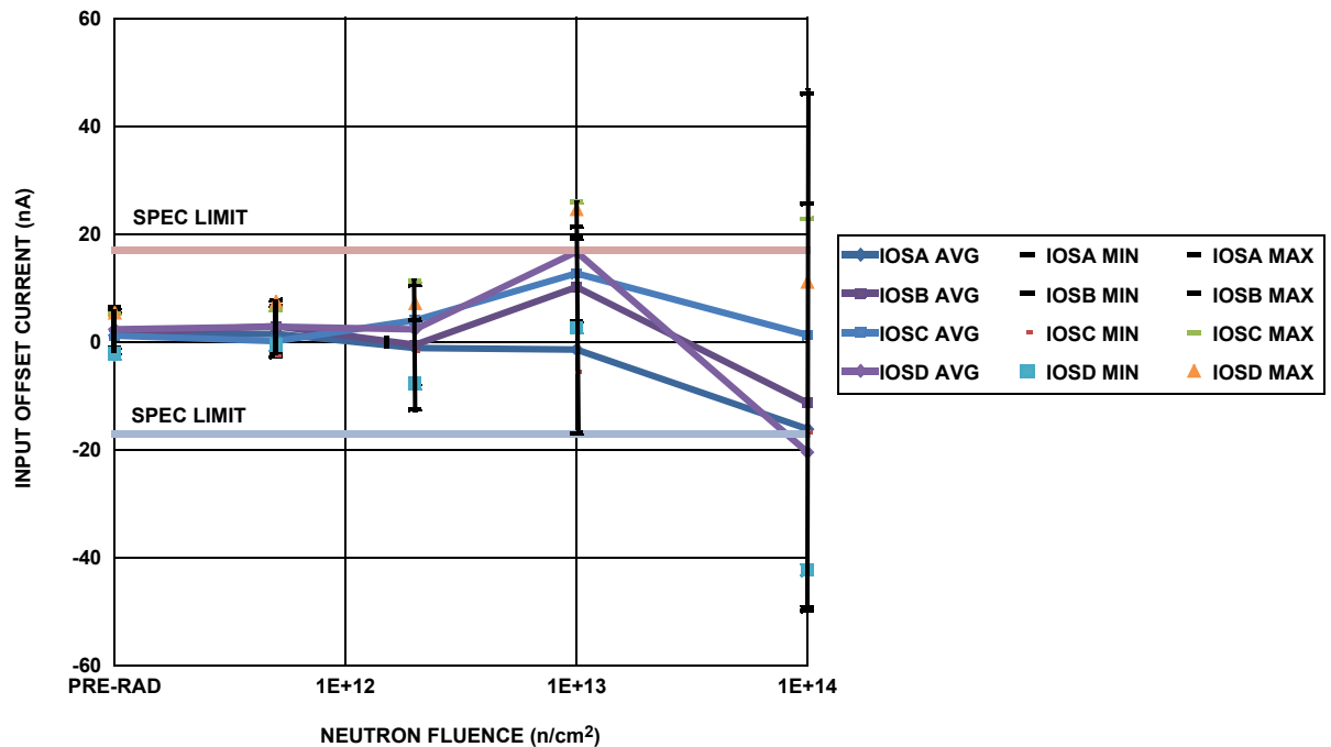
Figure 5. ISL70444SEH input offset current as a function of neutron irradiation, each channel, showing the mean, minimum and maximum of the populations at each level. Sample size was 5 for each cell ( 5 \times 10^{11} \text{ n/cm}^2 , 2 \times 10^{12} \text{ n/cm}^2 , 1 \times 10^{13} \text{ n/cm}^2 and 1 \times 10^{14} \text{ n/cm}^2 ), with two control units. The post-total dose irradiation SMD limits are -17.0nA to +17.0nA.
