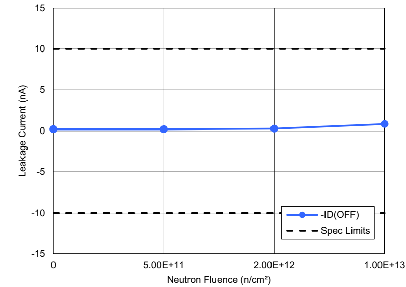
Figure 11. HS-508BEH negative OFF-drain leakage ( -I_{D(OFF)} ) following irradiation to each level. The error bars (if visible) represent the minimum and maximum measured values. The post-TID irradiation SMD limits are a minimum of -10nA and a maximum of 10nA.
