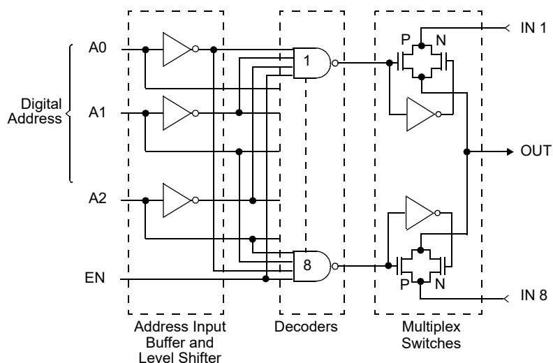
Figure 1. HS-508BEH, HS-508BRH Function Block Diagram
