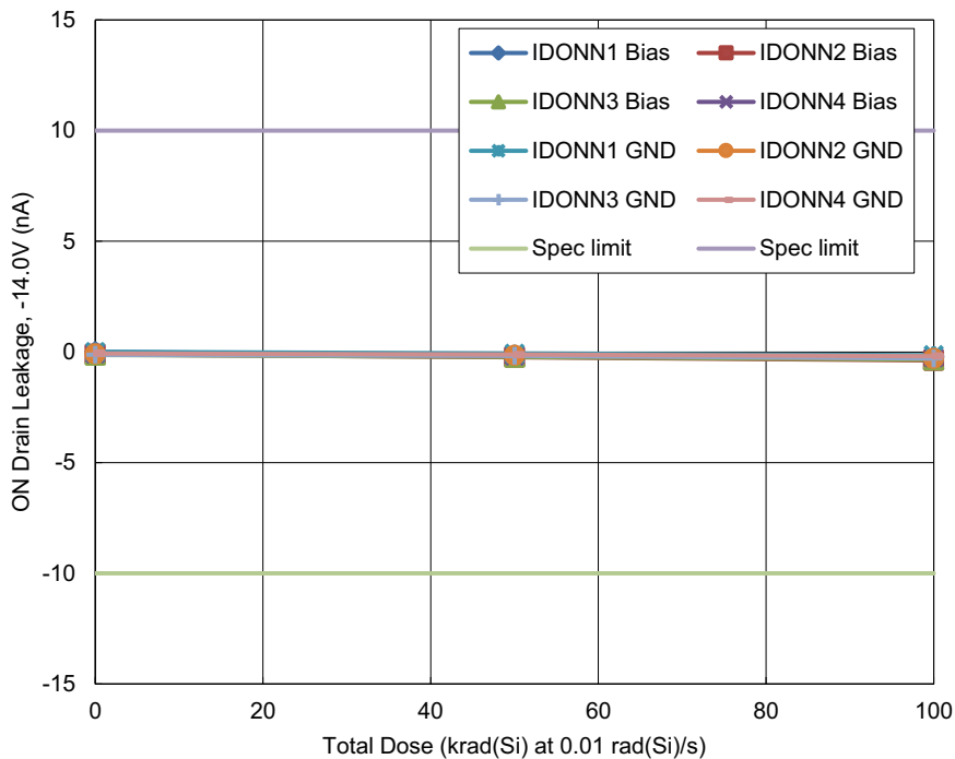
Figure 11. HS-201HSEH ON drain leakage at -14.0V, each channel, as a function of LDR total dose irradiation for the biased and unbiased (all pins grounded) cases. The dose rate was 0.01rad(Si)/s. The sample sizes for the two LDR cells were 30 for each cell. The specification limits are -10.0nA to +10.0nA.
