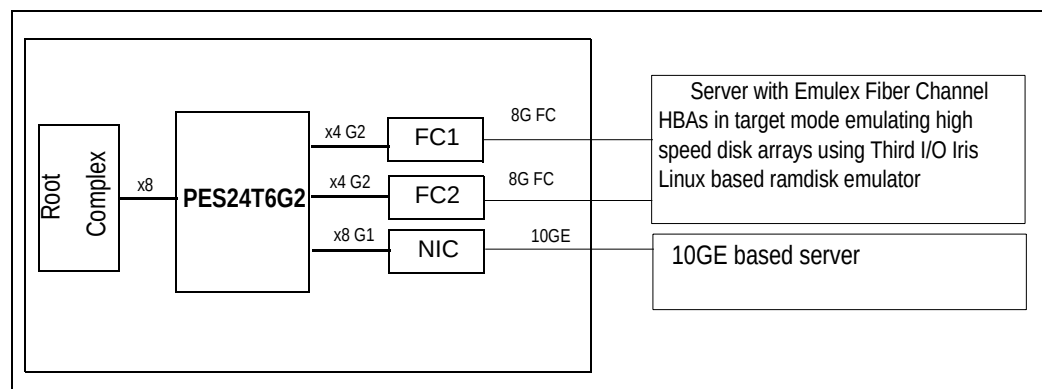
Figure 7 FC &amp; GE Throughput Measurement Setup with the PES24T6G2 and two Fiber Ports
