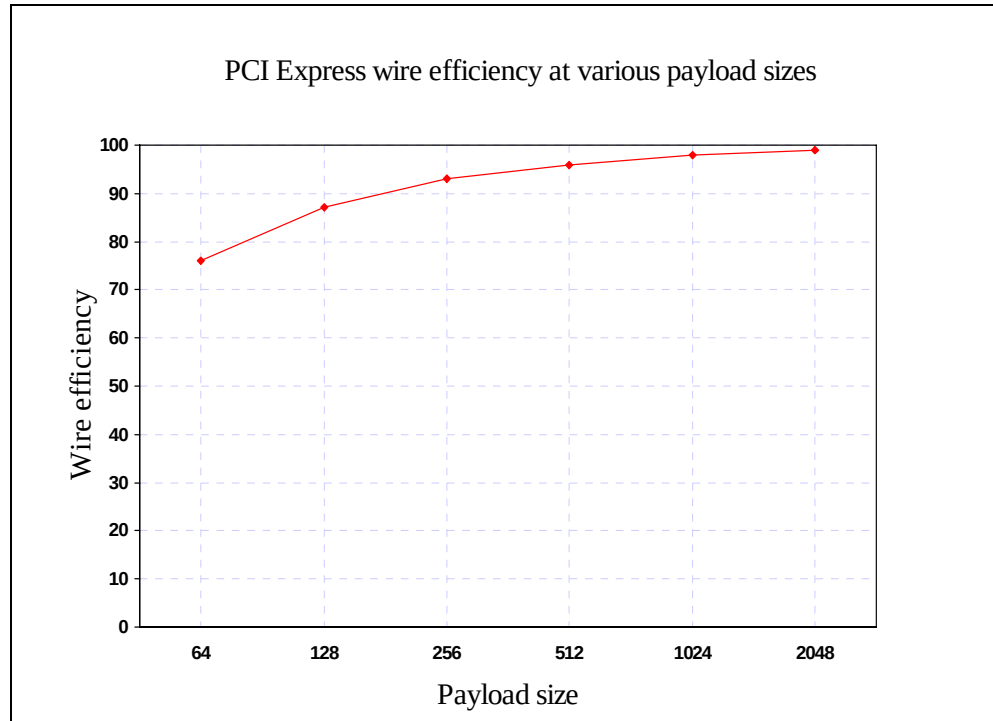
Figure 3 Data Path Efficiency of a PCI Express Link
