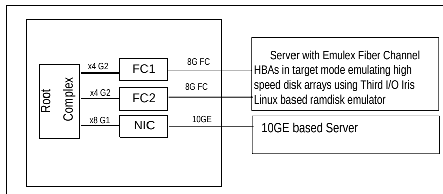
Figure 8 FC and GE Throughput Measurement without the PES24T6G2 and Two Fiber Ports
