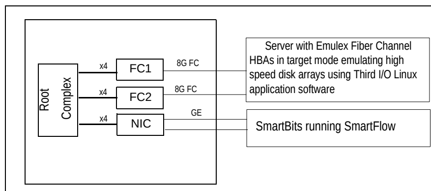
Figure 10 FC &amp; GE Throughput Measurement without the PES24T6G2
