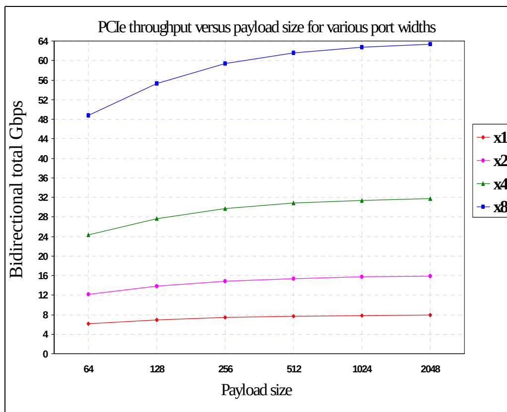
Figure 2 Effect of Framing Overhead on Link Efficiency
