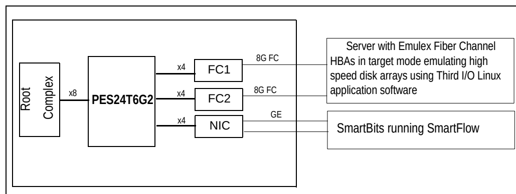
Figure 9 FC & GE Throughput Measurement Setup with the PES24T6G2
