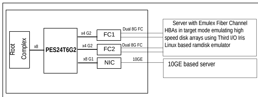
Figure 5 FC & GE Throughput Measurement Setup with the PES24T6G2 and 4 Fiber Ports
