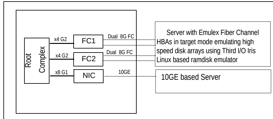
Figure 6 FC &amp; GE Throughput Measurement without the PES24T6G2 and 4 Fiber Ports
