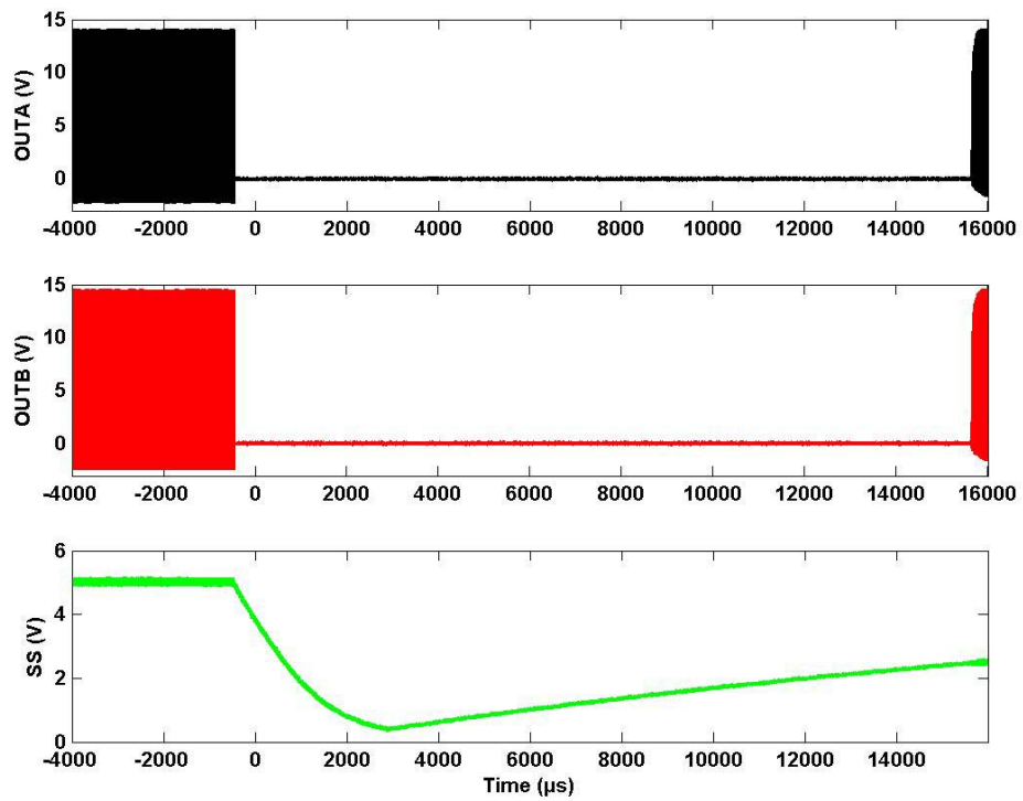
Figure 5. First SEFI for DUT2 Irradiated with 86.3\text{MeV}\cdot\text{cm}^2/\text{mg} Gold
