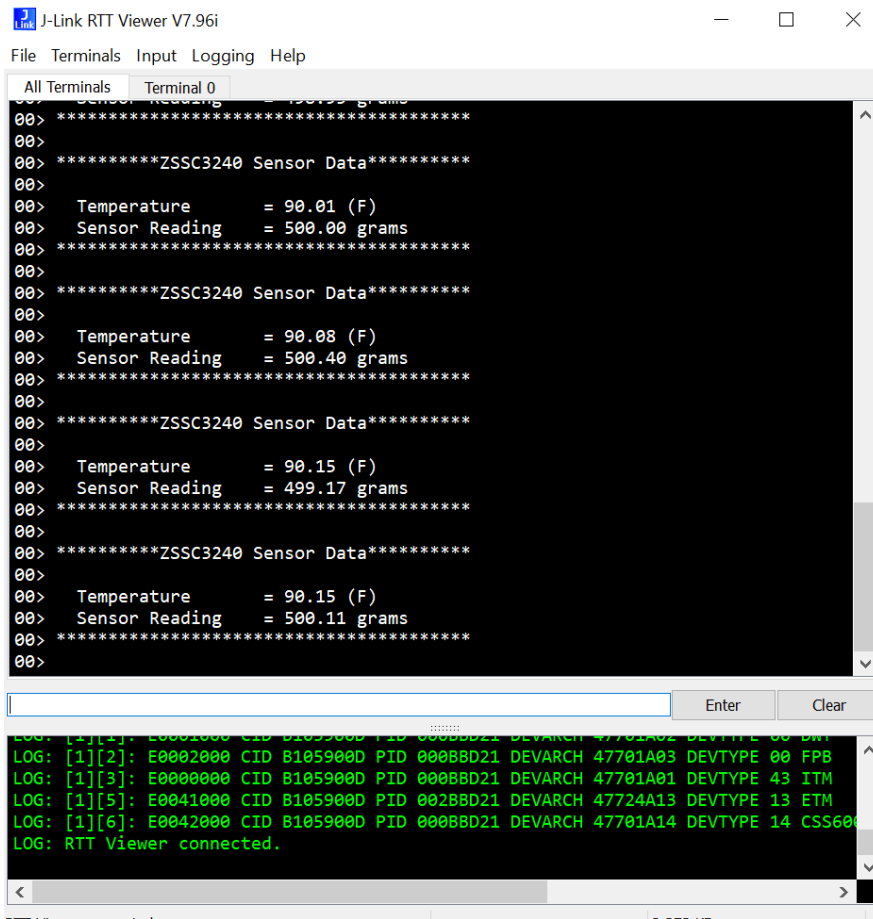
Figure 15. Sensor Output with 500g Weight
