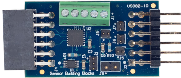
Figure 1. US082-SSC3240EVZ Board
