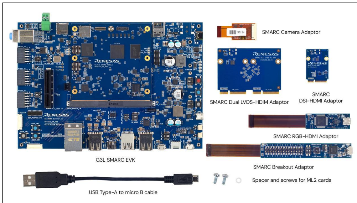
Figure 1. RZ/G3L Evaluation Board Kit Contents
