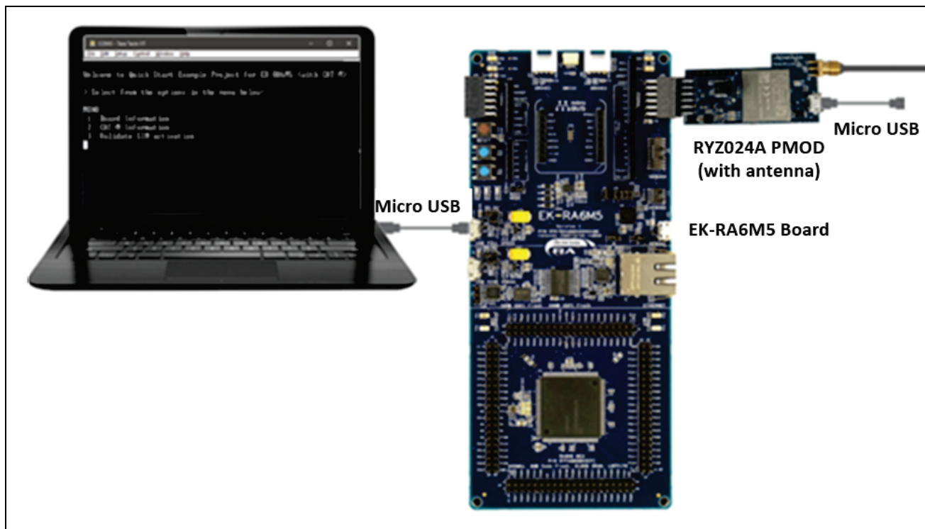
Figure 4. Connecting the EK-RA6M5 Board to the Host PC via USB Full Speed Port
