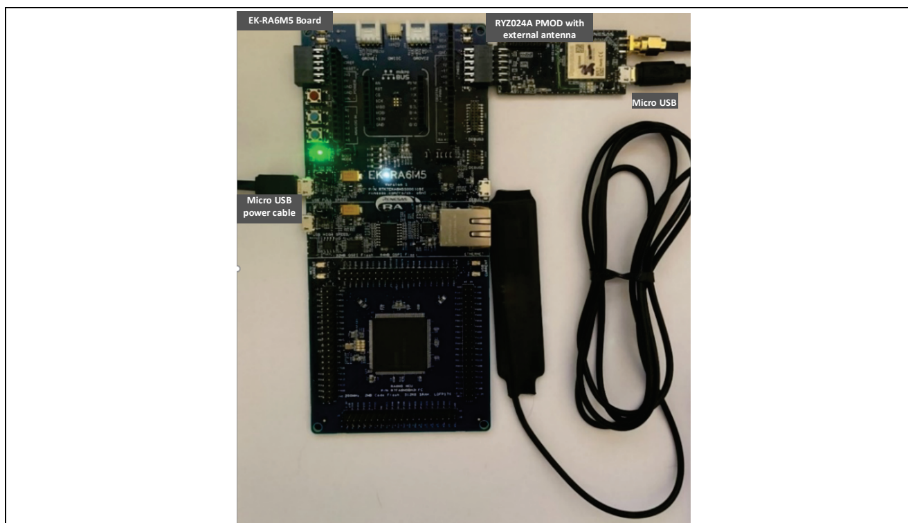
Figure 1. EK-RA6M5 Setup with RYZ024A PMOD Board Connected
