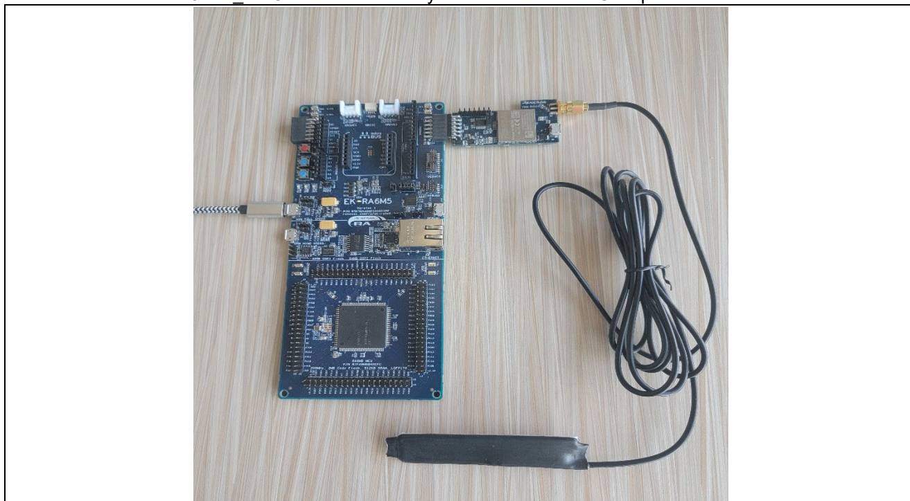
Figure 1. EK-RA6M5 Setup with RYZ014A_PMOD Module Connected
