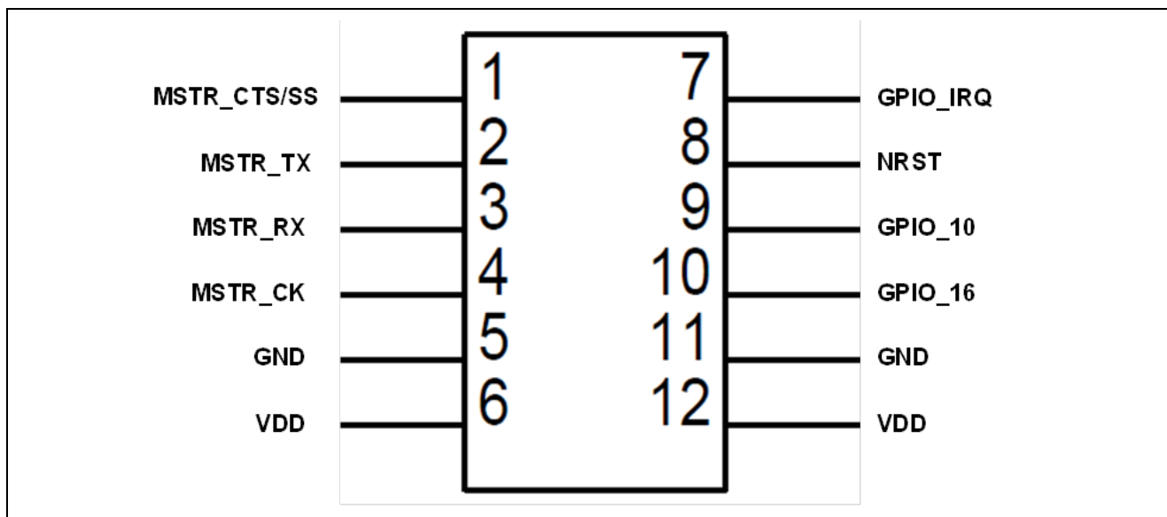
Figure 1. Pin Diagram
