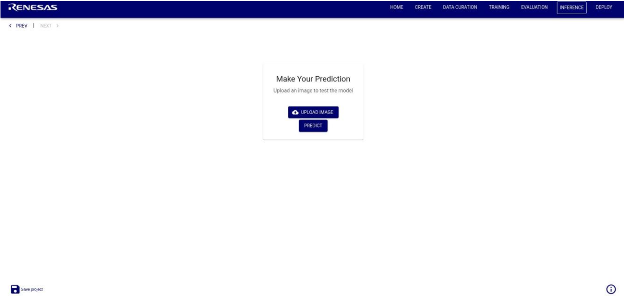
Figure 11: Inference Page
