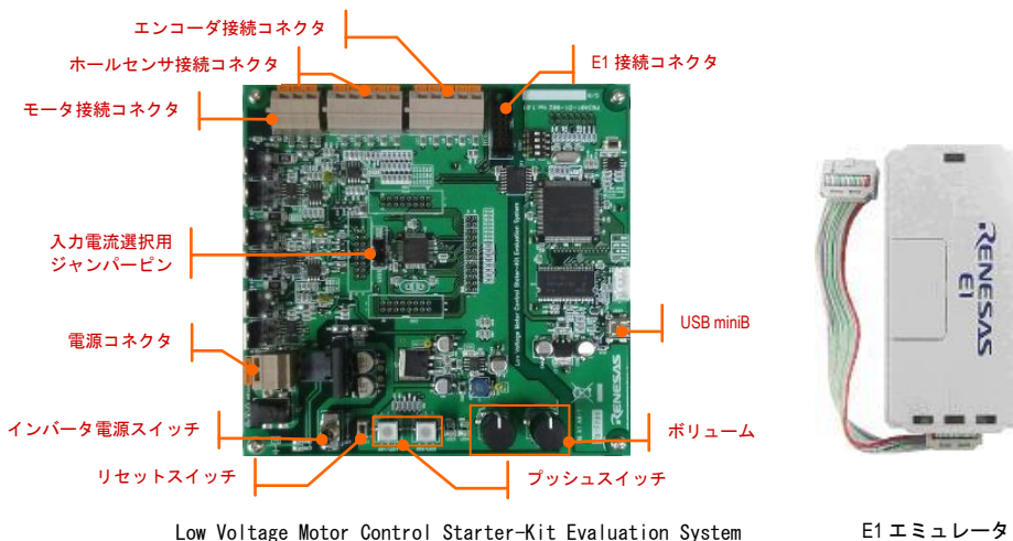
Low Voltage Motor Control Starter-Kit Evaluation System
