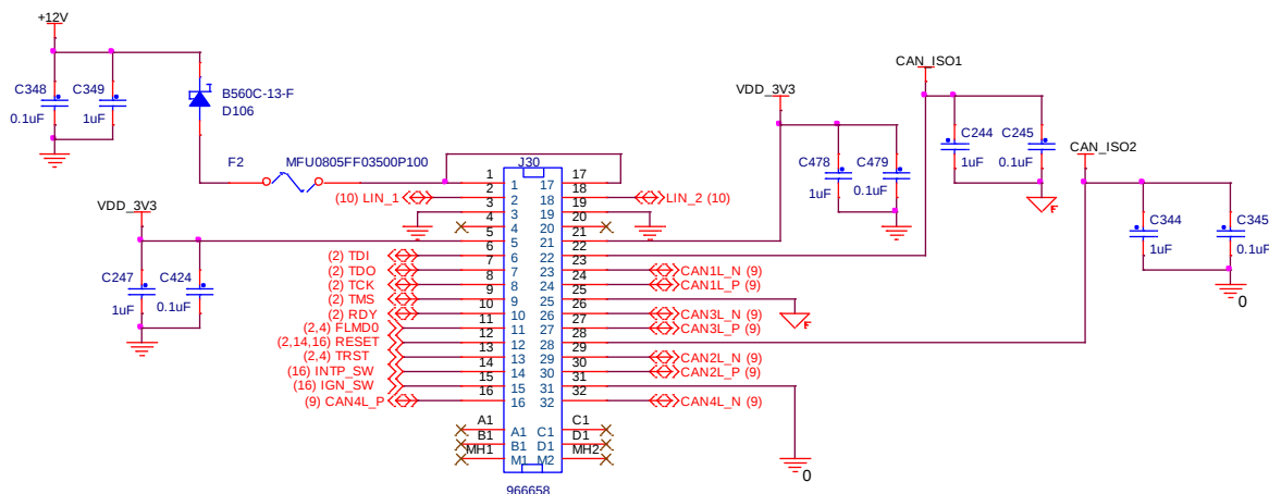
Figure 4-19 Main connector
