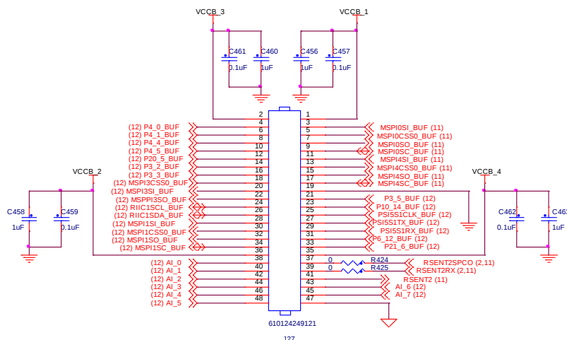
Figure 4-18 I/O connector
