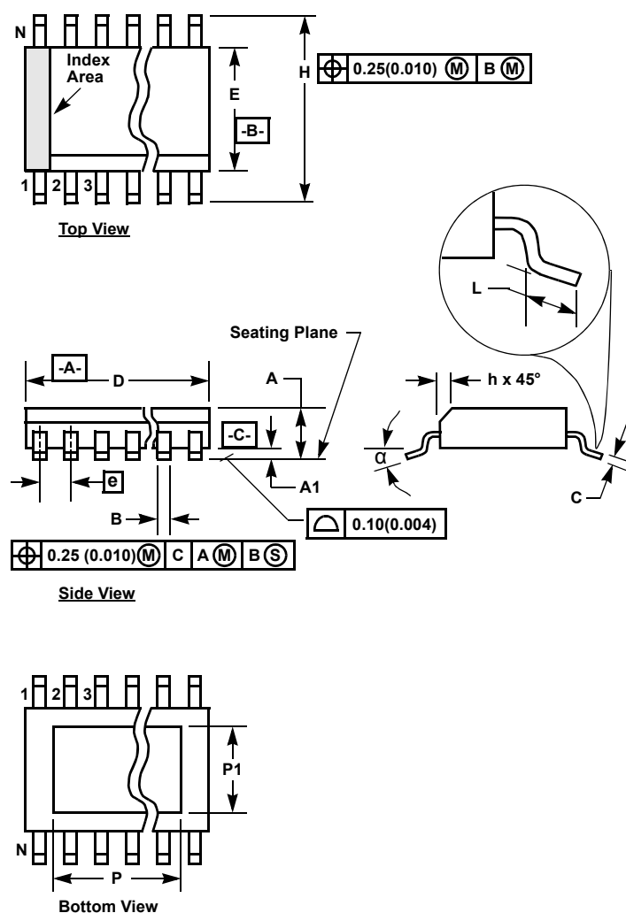
M8.15C 8 Lead Narrow Body Small Outline Exposed Pad Plastic Package (EPSONIC)
