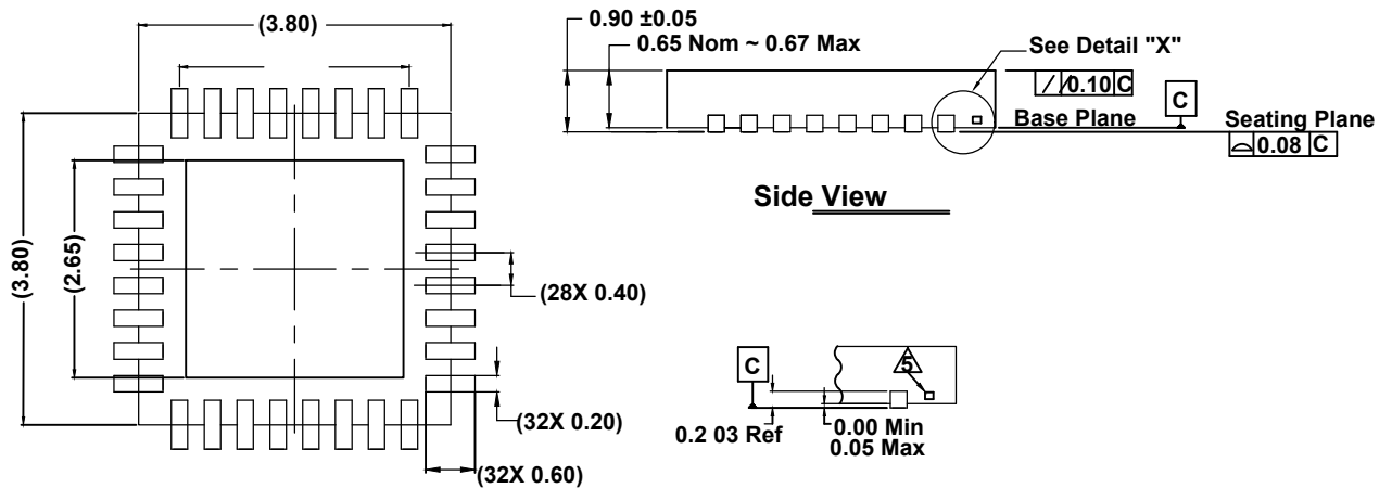
Typical Recommended Land Pattern
