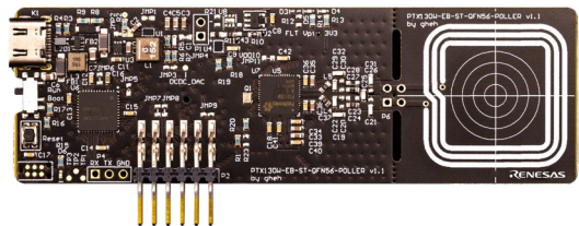
WLC Poller (PTX130W) board
