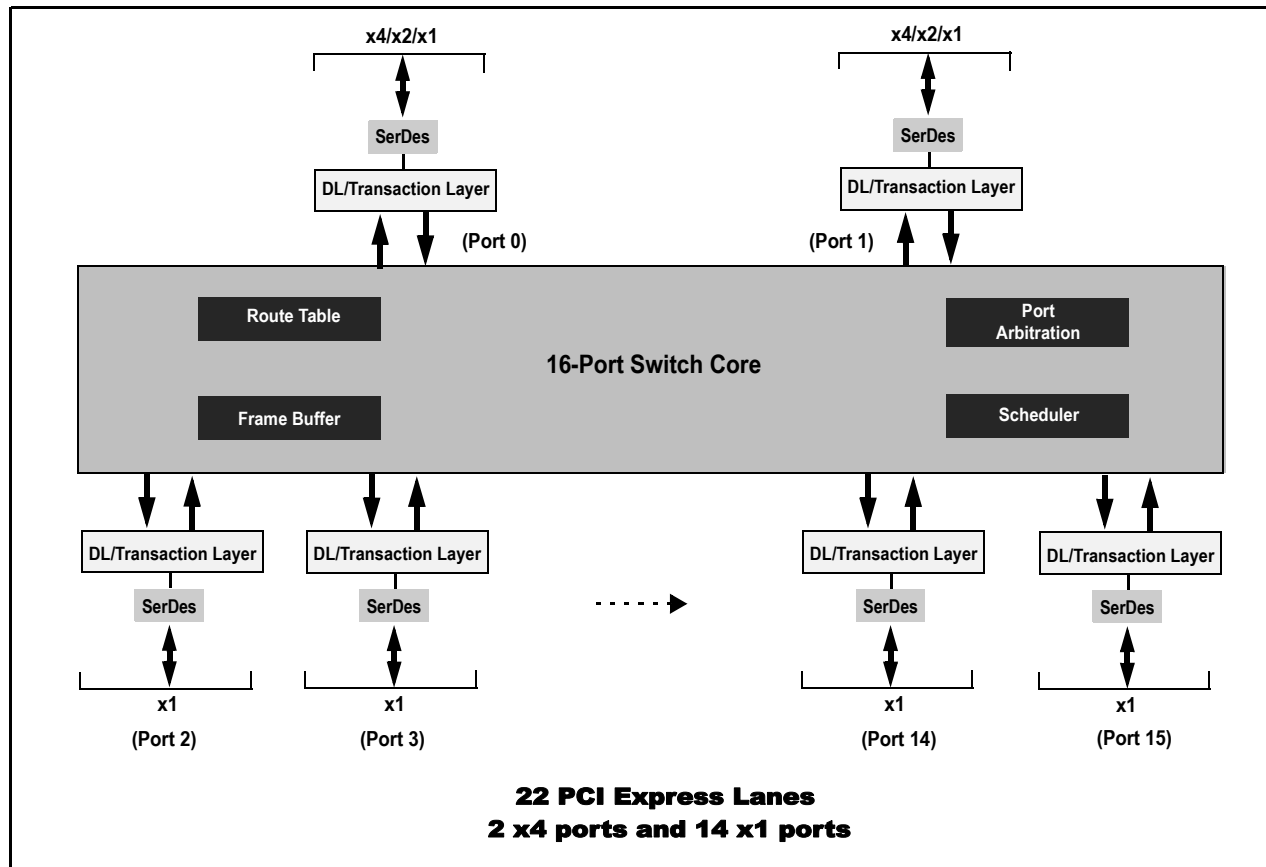
Figure 1 PES22H16G2 Block Diagram
