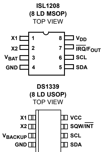
FIGURE 1. PACKAGE PINOUTS
