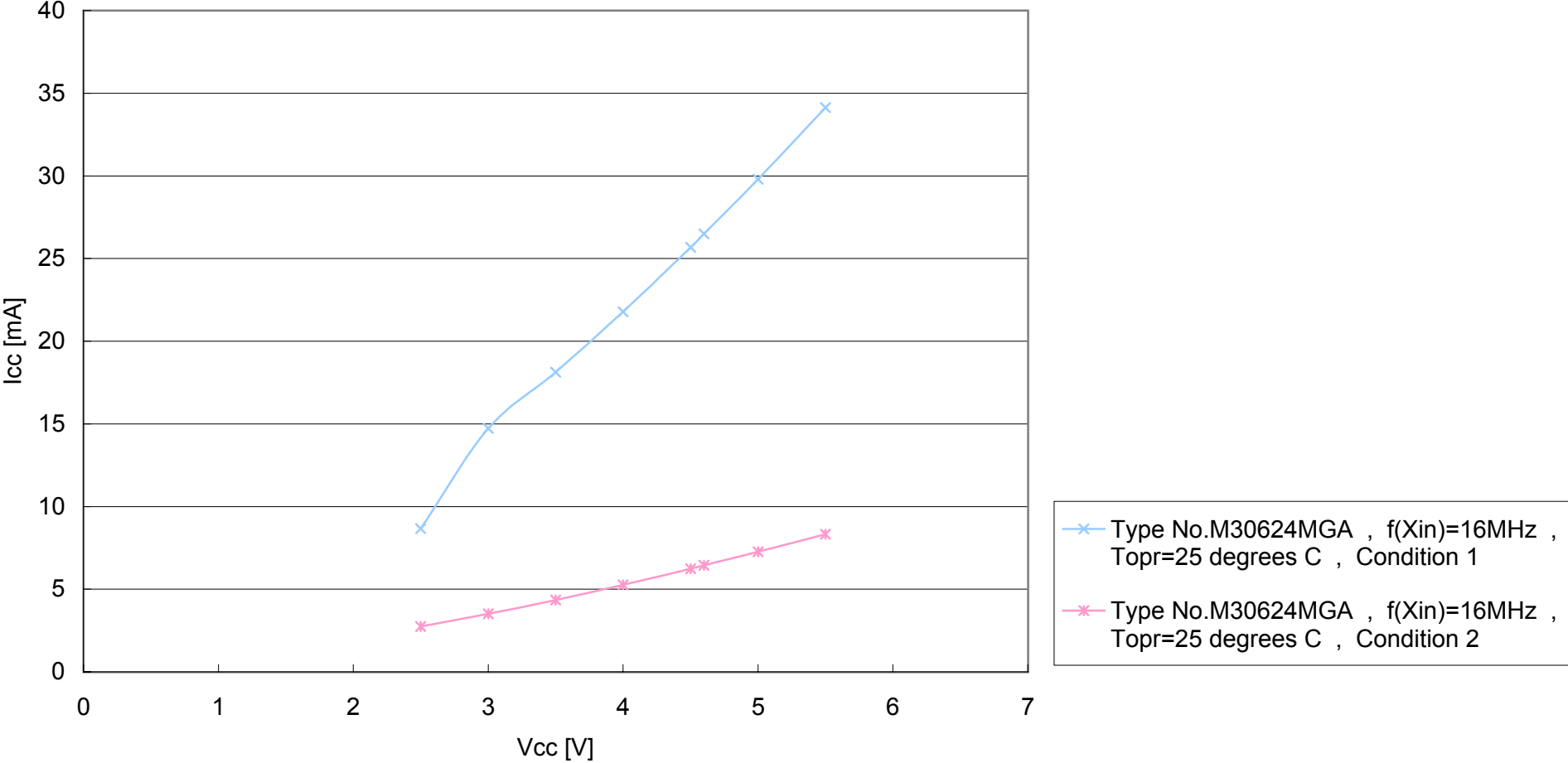
Vcc-Icc (Normal Operation Mode)
