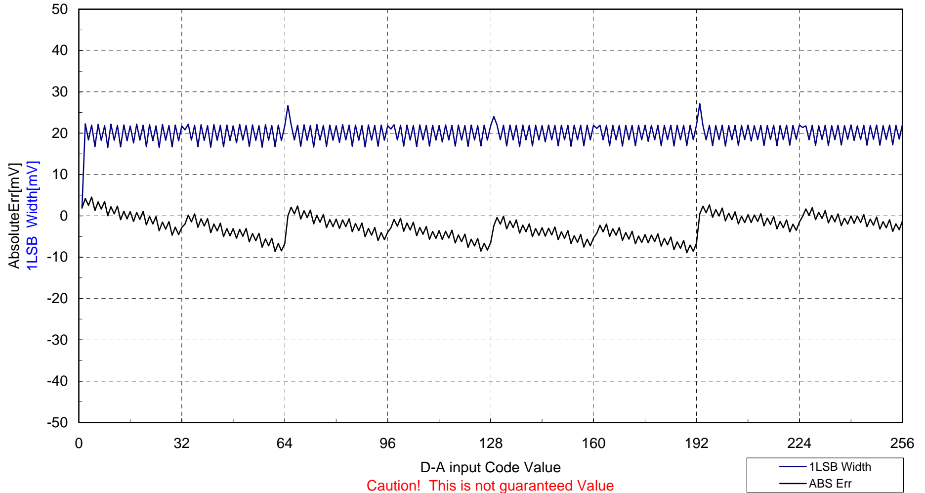
M30624FGAFP D-A Accuracy Condition : AVcc=Vcc=Vref=5.12V,f(Xin)=16.0MHz,Topr=25 degrees C, 1LSB-Width = 20mV
