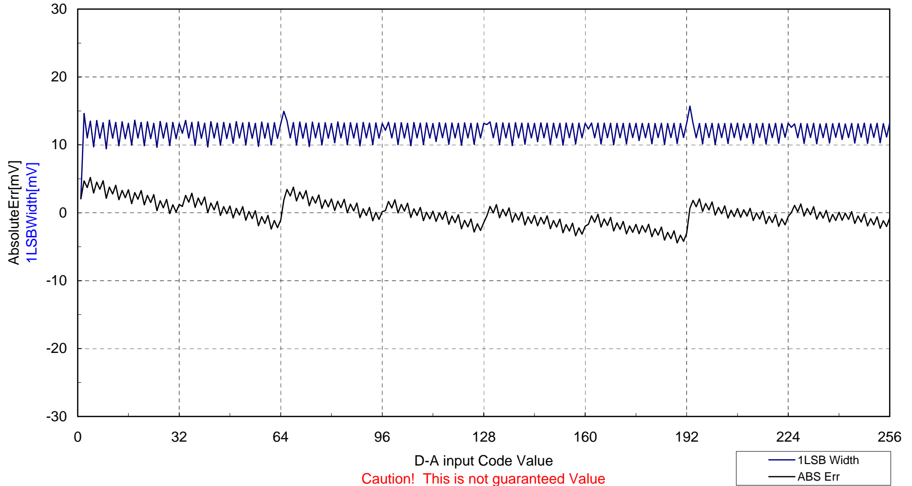
M30624FGAFP D-A Accuracy Condition : AVcc=Vcc=Vref=3.072V,f(Xin)=7.0MHz,Topr=25 degrees C, 1LSB-Width = 12mV
