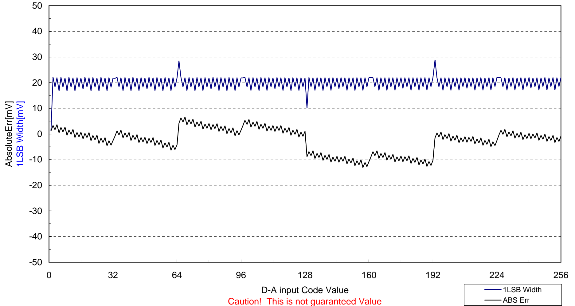
M30620MCAFP D-A Accuracy Condition : AVcc=Vcc=Vref=5.12V, f(Xin)=16.0MHz, Topr=25 degrees C, 1LSB-Width = 20mV
