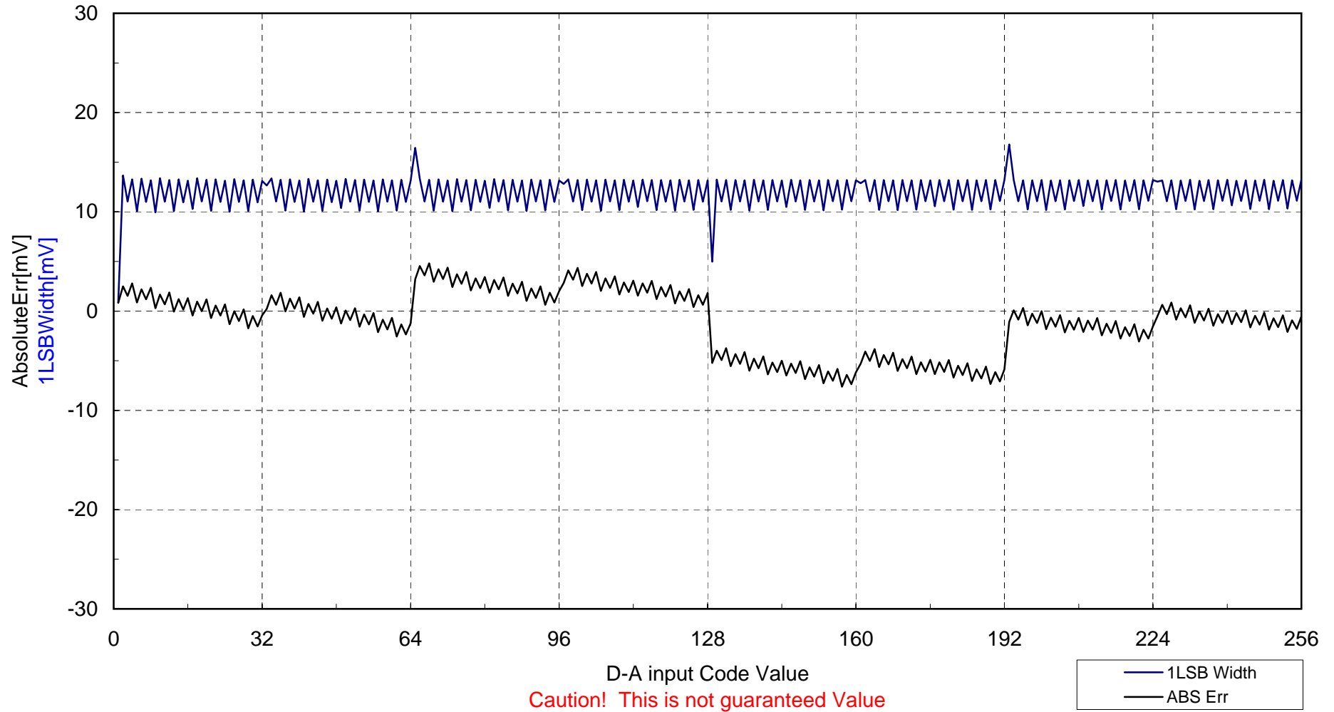
M30620MCAFP D-A Accuracy Condition : AVcc=Vcc=Vref=3.072V, f(Xin)=7.0MHz, Topr=25 degrees C, 1LSB-Width = 12mV
