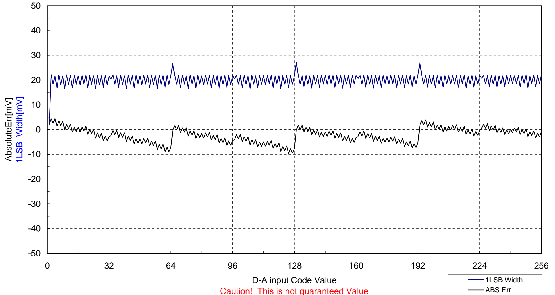
M30620FCAFP D-A Accuracy Condition : AVcc=Vcc=Vref=5.12V,f(Xin)=16.0MHz,Topr=25 degrees C, 1LSB-Width = 20mV
