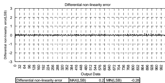
Figure28. Topr=25(degrees C)
