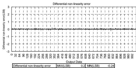
Figure27. Topr=-40(degrees C)
