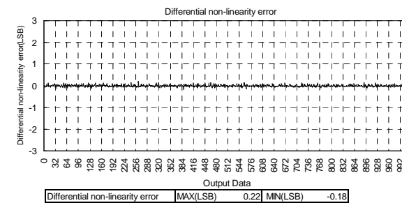
Figure29. Topr=85(degrees C)
