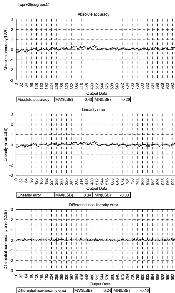
Figure19. Topr=25(degrees C)
