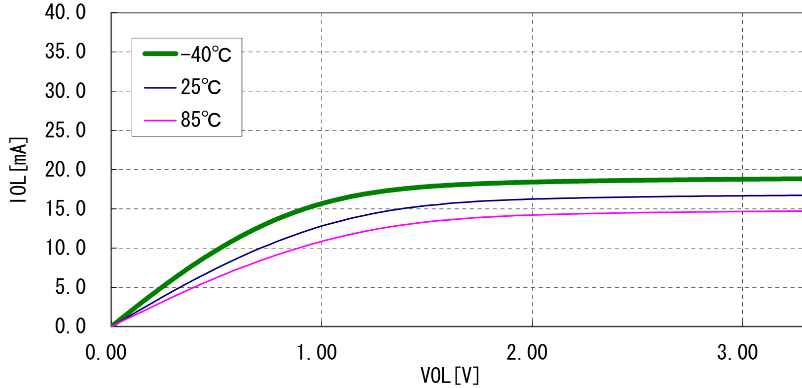
R32C/116, 117, 118 Group CMOS Port VOL Vcc=3.3V
