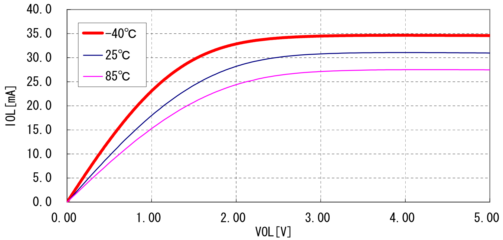
R32C/116, 117, 118 Group CMOS Port VOL Vcc=5V
