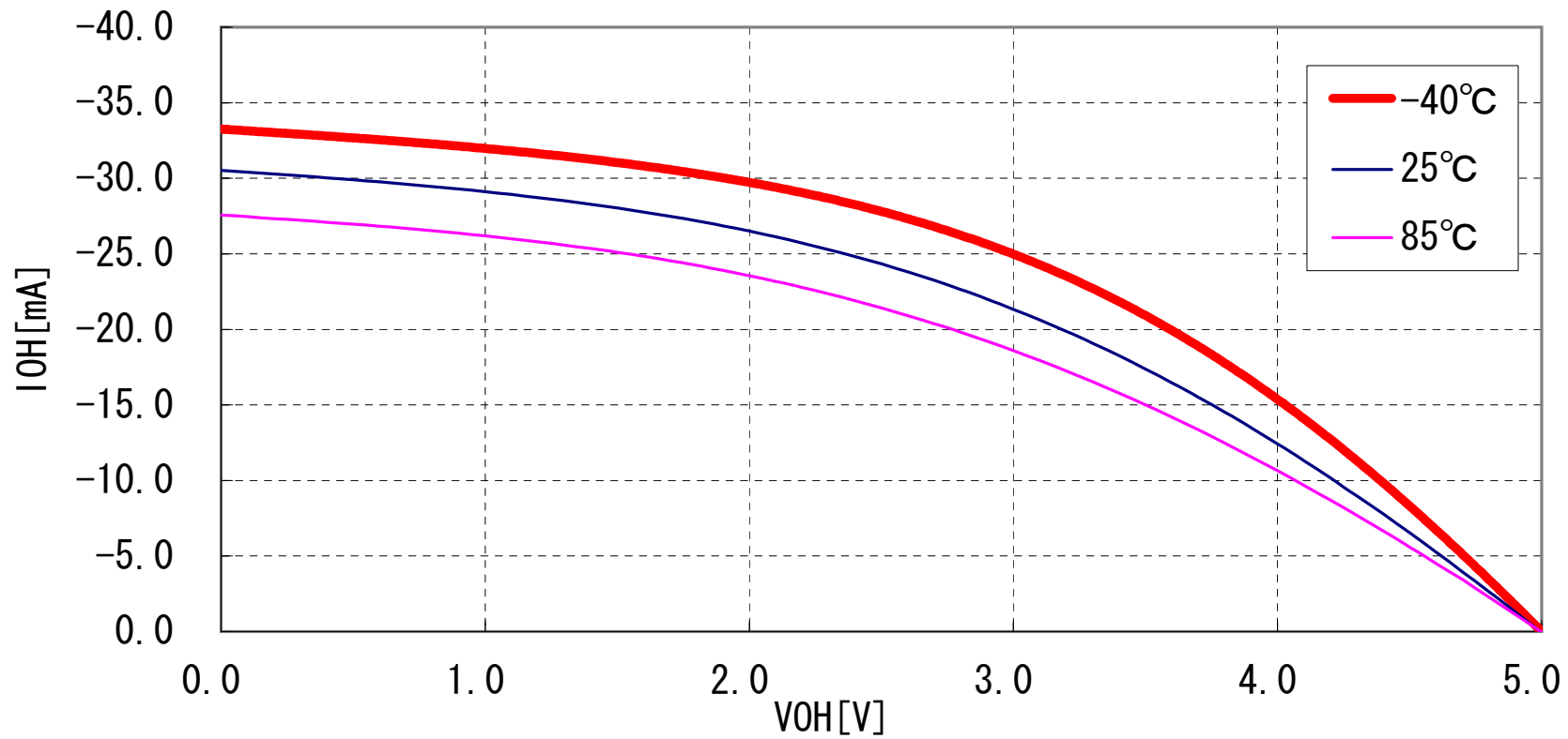
R32C/116, 117, 118 Group CMOS Port VOH Vcc=5V
