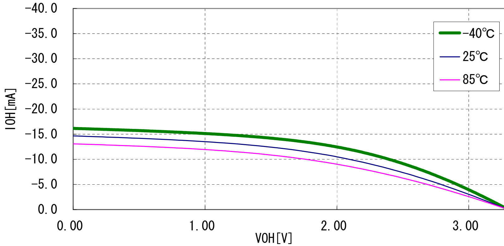
R32C/116, 117, 118 Group CMOS Port VOH Vcc=3.3V
