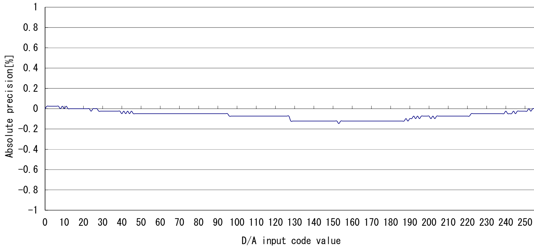
R32C/116, 117, 118 Group D/A Accuracy (V cc =A vcc =V ref =5V, T a =25°C, Resolution=8bits)
