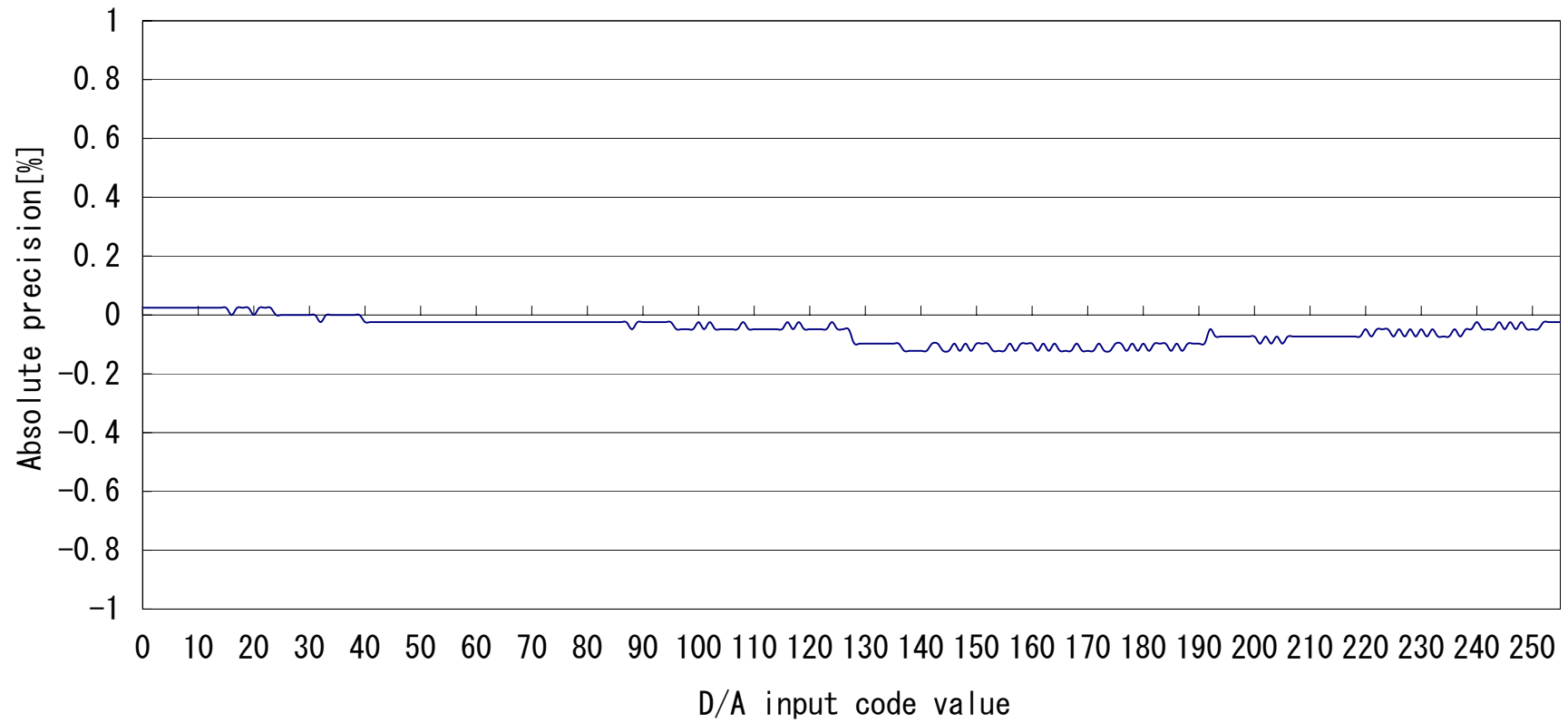
R32C/116, 117, 118 Group D/A Accuracy ( V_{CC}=A_{VCC}=V_{REF}=3.3V , T_a=25^{\circ}C , Resolution=8bits)
