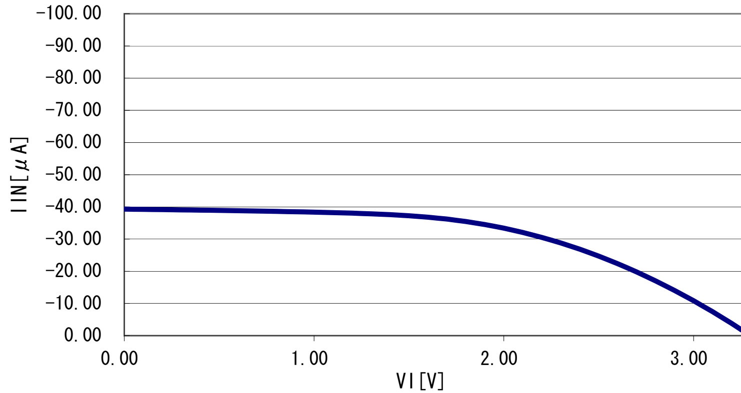
R32C/116, 117, 118 Group Pull-up resistor Vcc=3.3V, Ta=25°C
