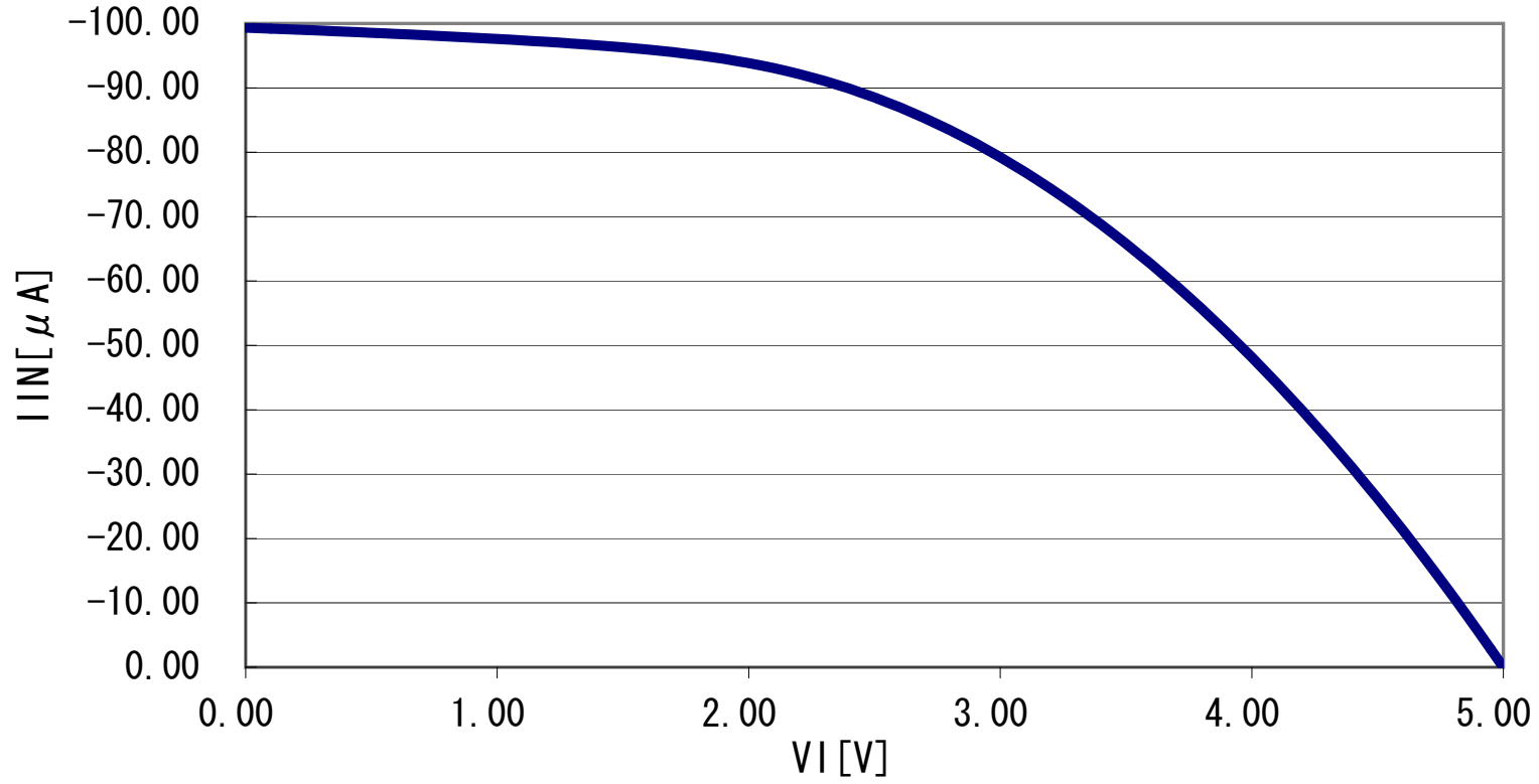
R32C/116, 117, 118 Group Pull-up resistor Vcc=5V, Ta=25°C
