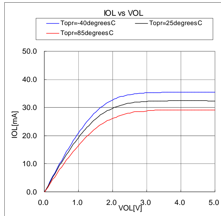
Figure12. IOL vs VOL (Vcc=5.0V)
