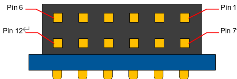
Figure 4. PMOD connector
