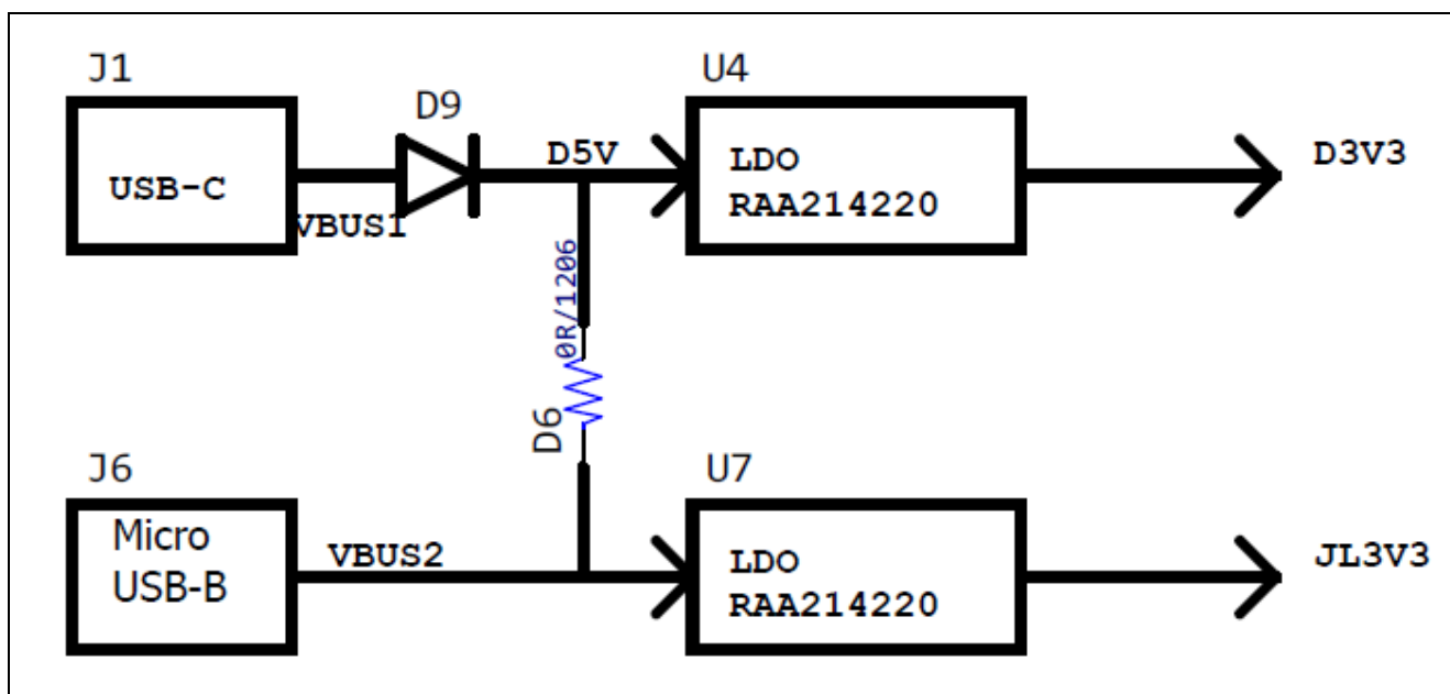
Figure 5. VOICE-RA6E1 Power Block Diagram
