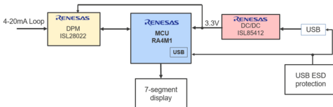
Figure 2. Block Diagram
