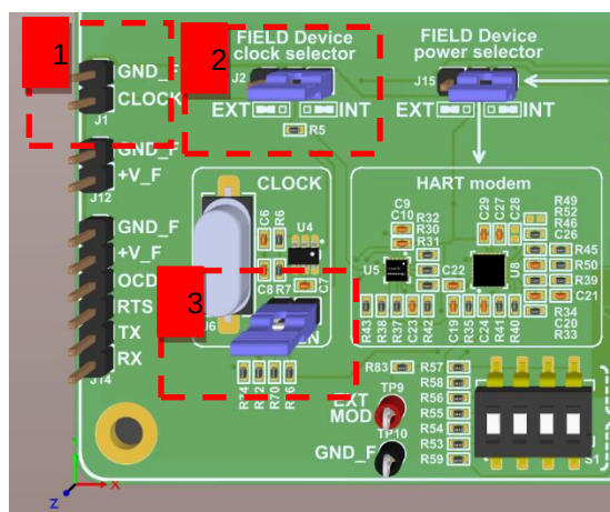
1– PINs for connecting external clock; 2 – clock selector; 3 – internal CLK enable
