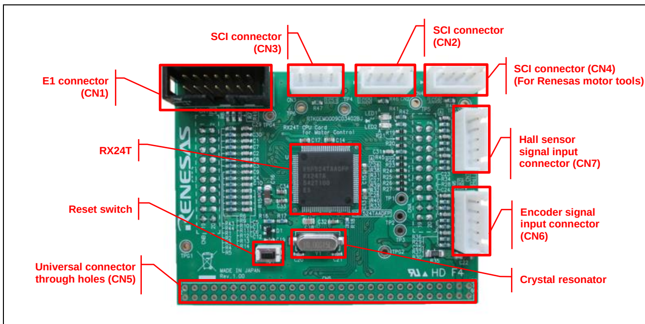
Figure 3.1 RX24T CPU Card Layout (Top view)
