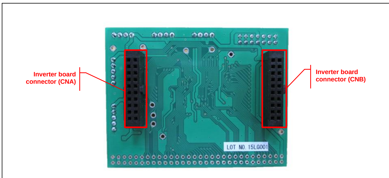
Figure 3.2 RX24T CPU Card Layout (Bottom view)
