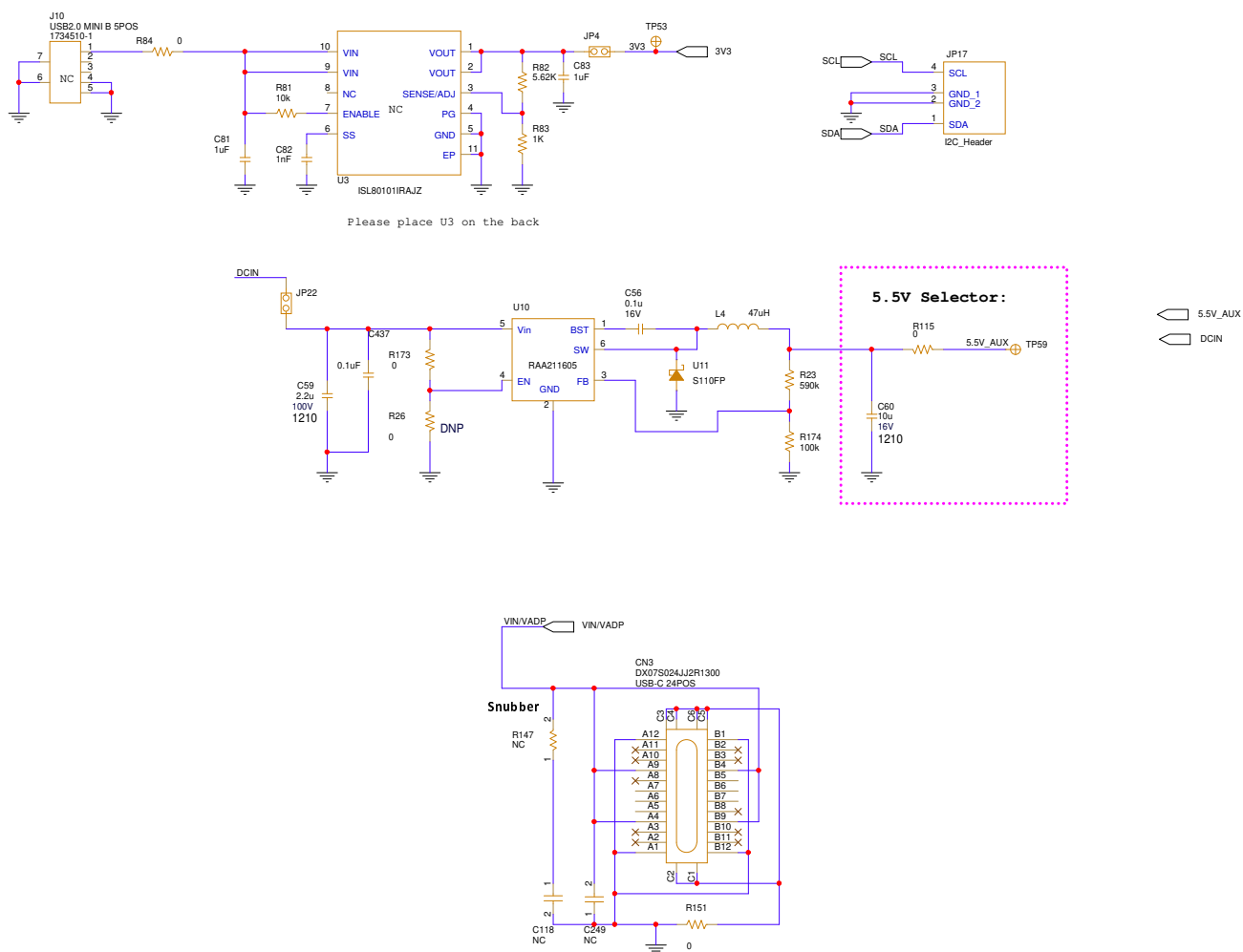
Figure 7. Schematic (2 of 2)
