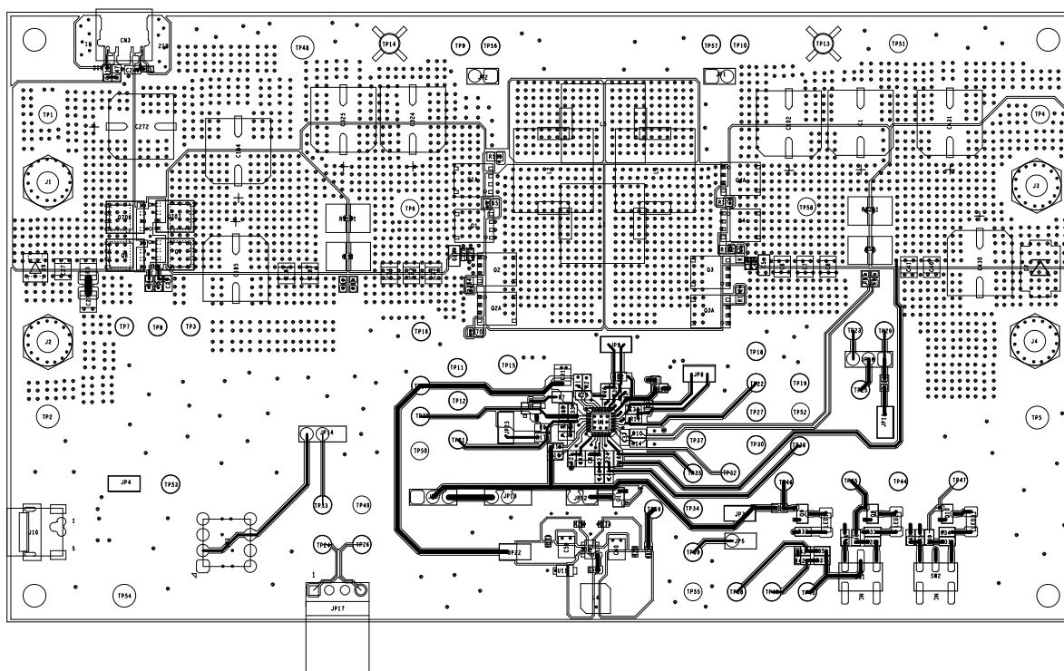
Figure 8. Top Layer
