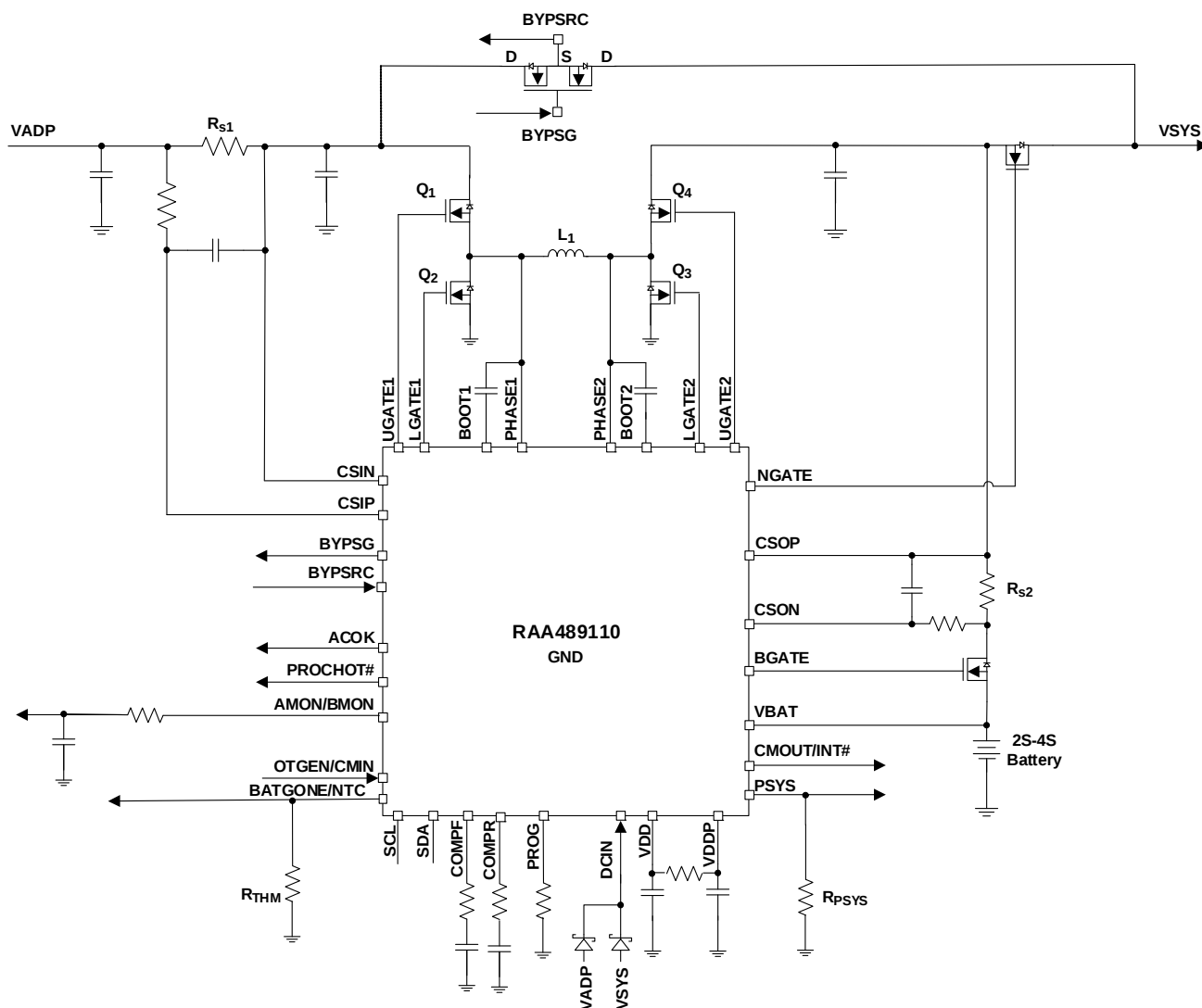
Figure 1. NVDC Plus HPBB Simplified Application Diagram
