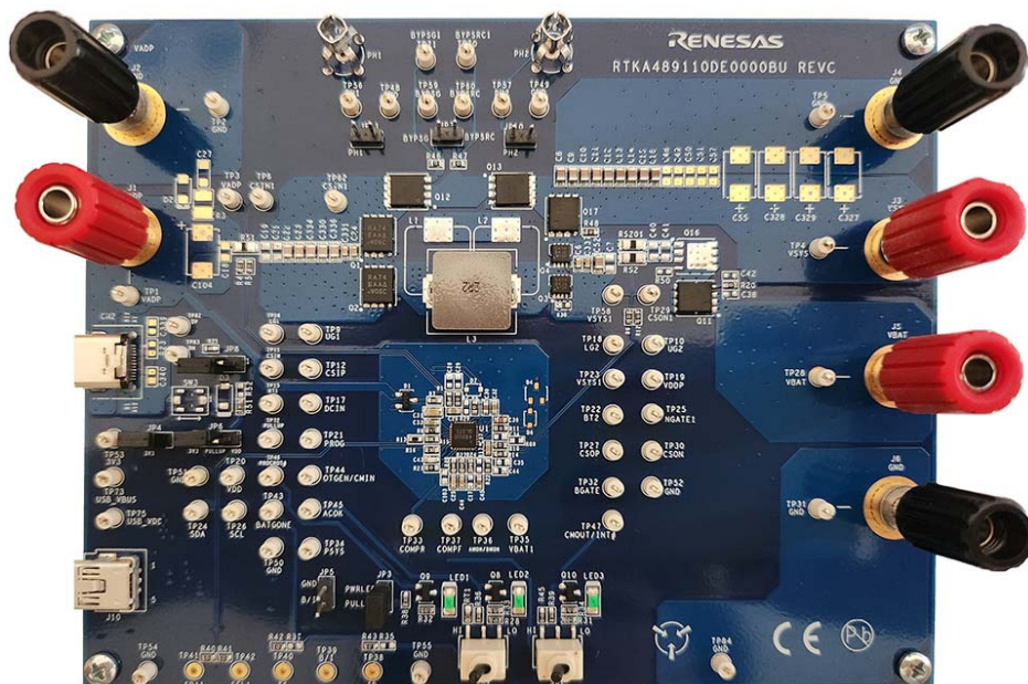
Figure 11. RTKA489110DE0000BU Evaluation Board (Top)
