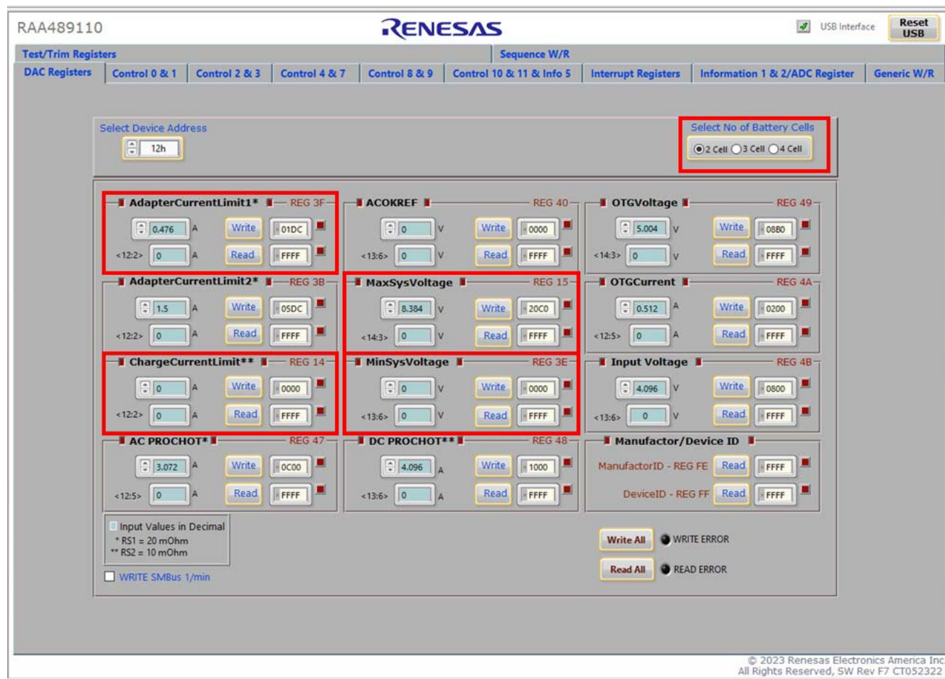
Figure 8. RAA489110 GUI
