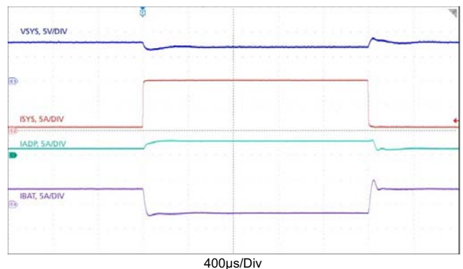
Figure 25. Buck Mode Transitions: Charge Current Loop to/from Adapter Current Loop. VADP = 20V, VBAT = 7V, MaxSystemVoltage = 8.384V, AdapterCurrentLimit = 3A, ChargeCurrent = 3A, SystemLoad: 0.5A \leftrightarrow 10A
