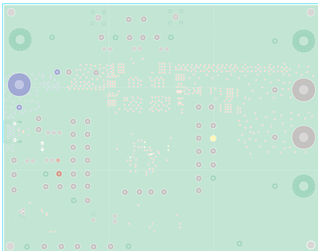
Figure 18. Inner Layer 4
