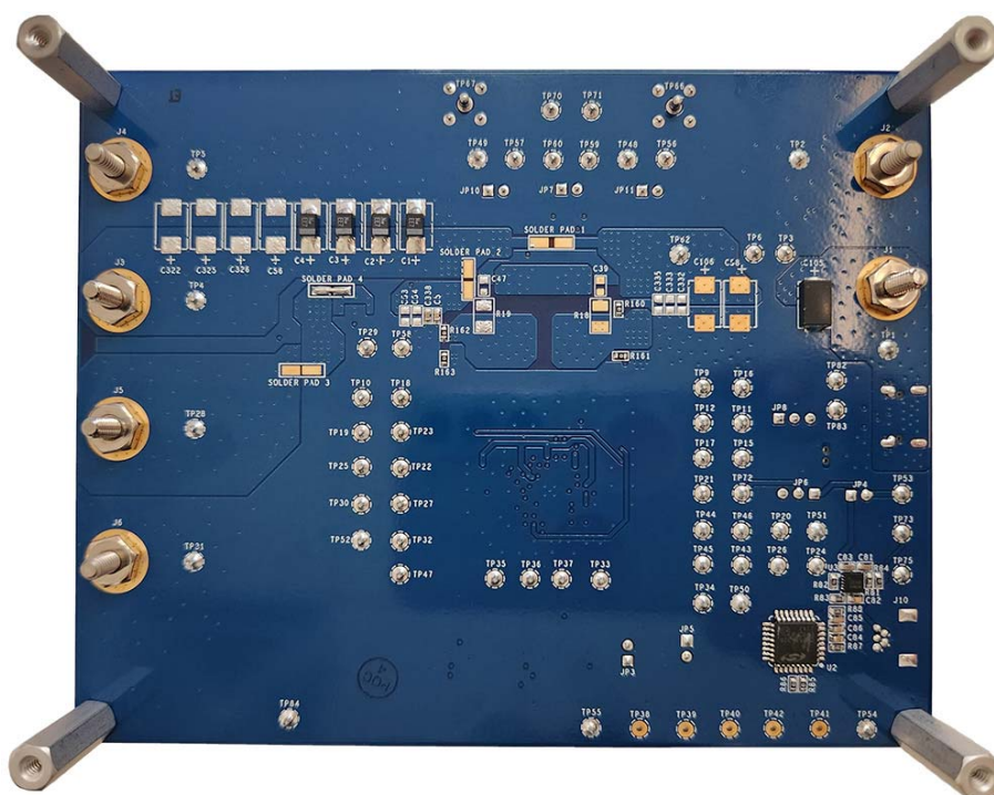
Figure 12. RTKA489110DE0000BU Evaluation Board (Bottom)
