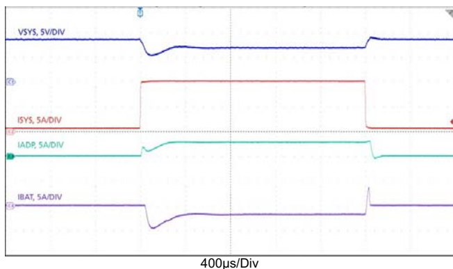
Figure 24. Buck Mode Transitions: Output Voltage Loop to/from Adapter Current Loop. VADP = 20V, VBAT = 7V, MaxSystemVoltage = 8.384V, AdapterCurrentLimit = 3A, ChargeCurrent = 0, SystemLoad: 0.5A \leftrightarrow 10A
