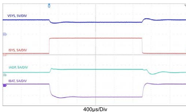
Figure 21. Boost Mode Transitions: Charge Current Loop to/from Adapter Current Loop. VADP = 5V, VBAT = 7V, MaxSystemVoltage = 8.384V, AdapterCurrentLimit = 3A, ChargeCurrent = 0.5A, SystemLoad: 0.5A <=> 8A
