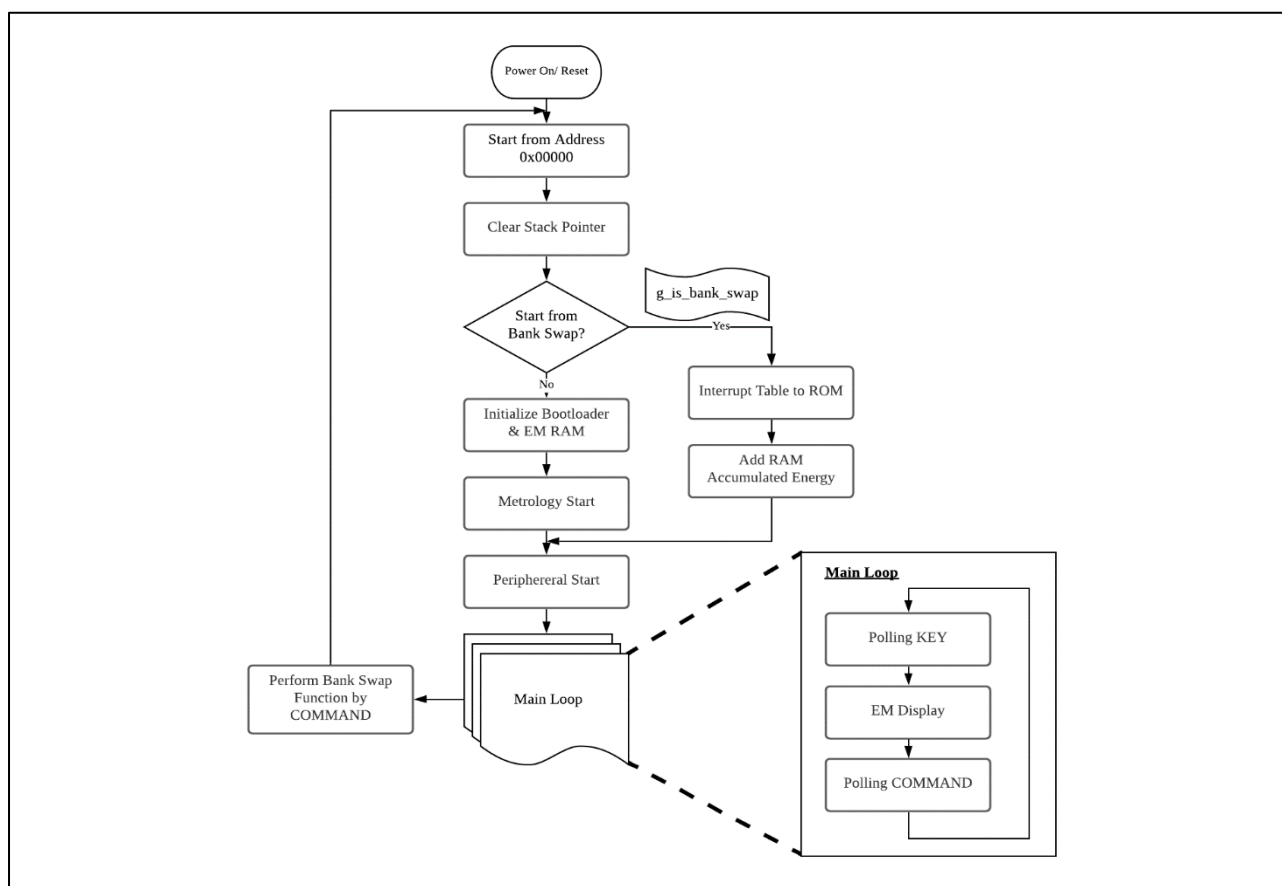
Figure 3: Continuous Metrology FOTA Project Flowchart
