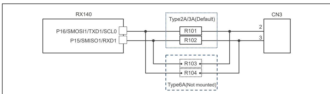
Figure 1-1. Pmod™ Interface Switch Circuit
