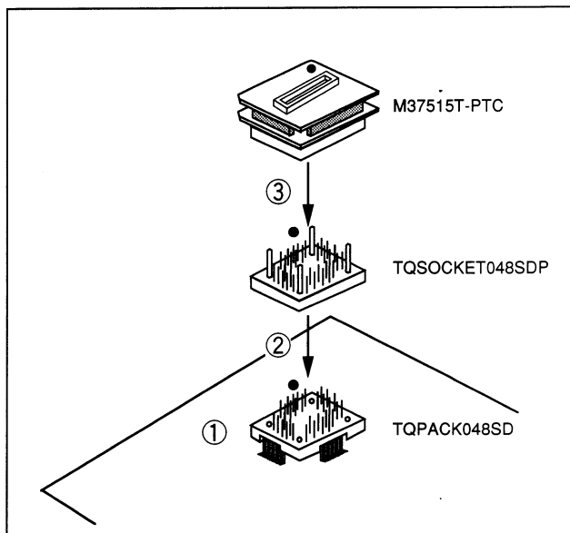
図3 M37515T-PTC装着手順
