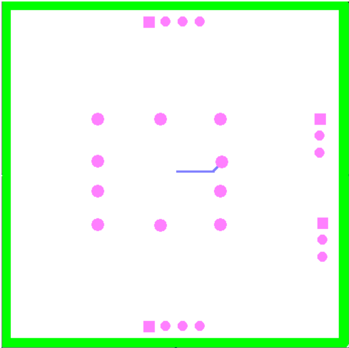
FIGURE 8. INNER LAYER 1
