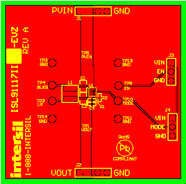
FIGURE 7. TOP LAYER
