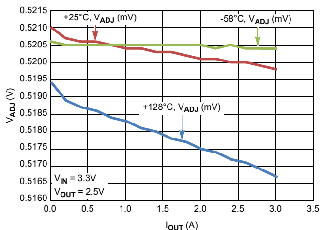
Figure 26. Load Regulation V_{ADJ} vs I_{OUT}
