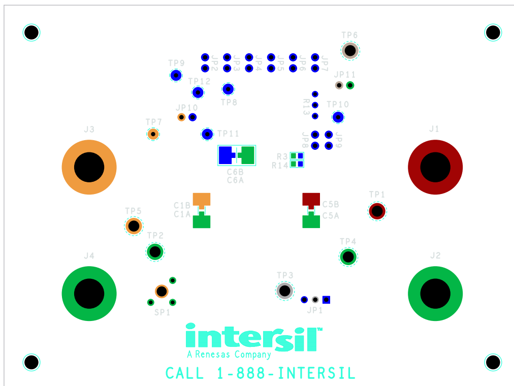
Figure 12. Silk Screen Bottom Mirror
