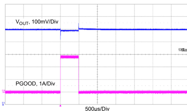
Figure 18. Load Transient, V_{IN} = 3.3V , V_{OUT} = 2.5V , C_{OUT} = 220\mu F 25m \Omega
