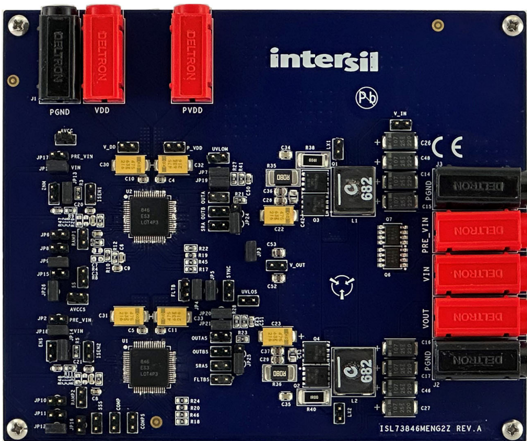
Figure 1. ISL73846MEV3Z 2-Phase Boost Converter Evaluation Board (Top)
