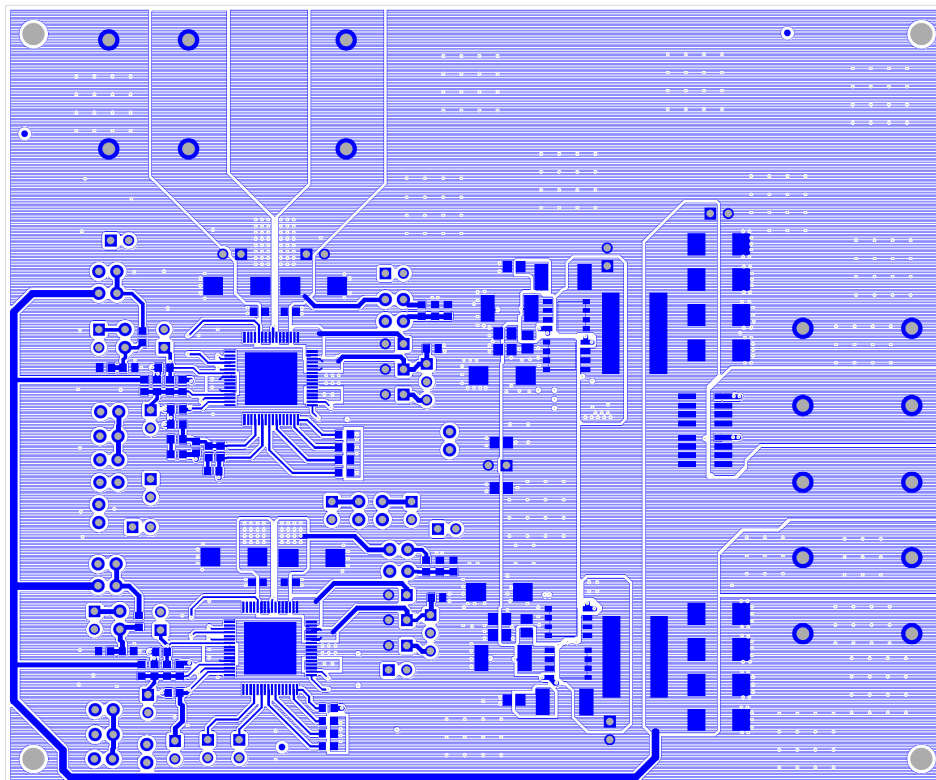
Figure 5. Top Layer
