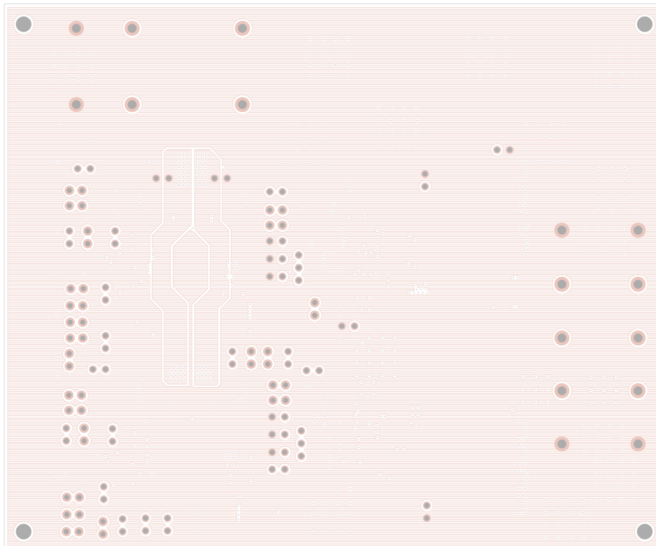
Figure 9. Layer 5
