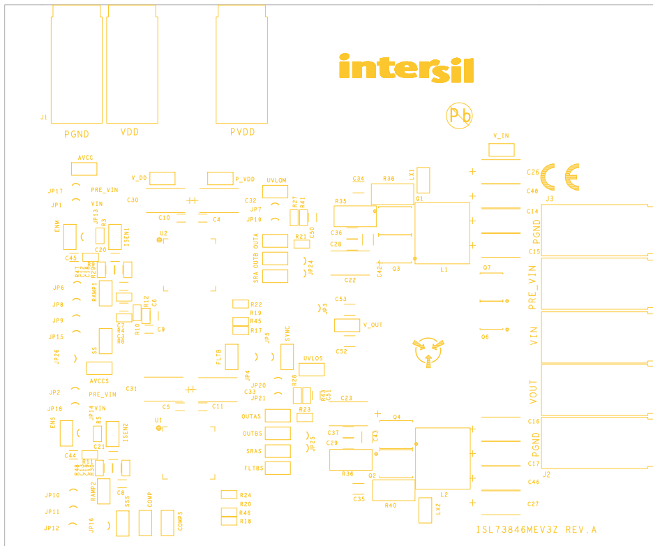
Figure 4. Silkscreen Top
