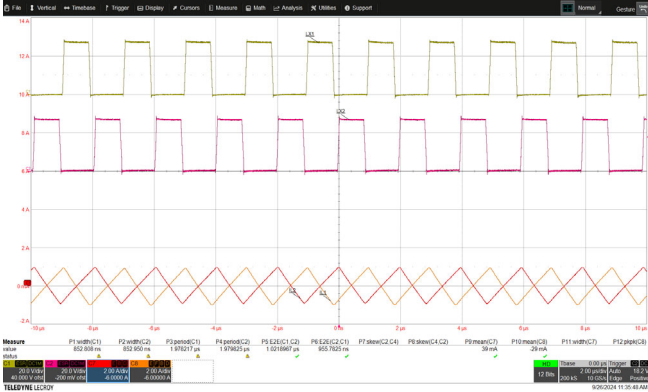
Figure 12. No Load LX Voltages and Inductor Currents
