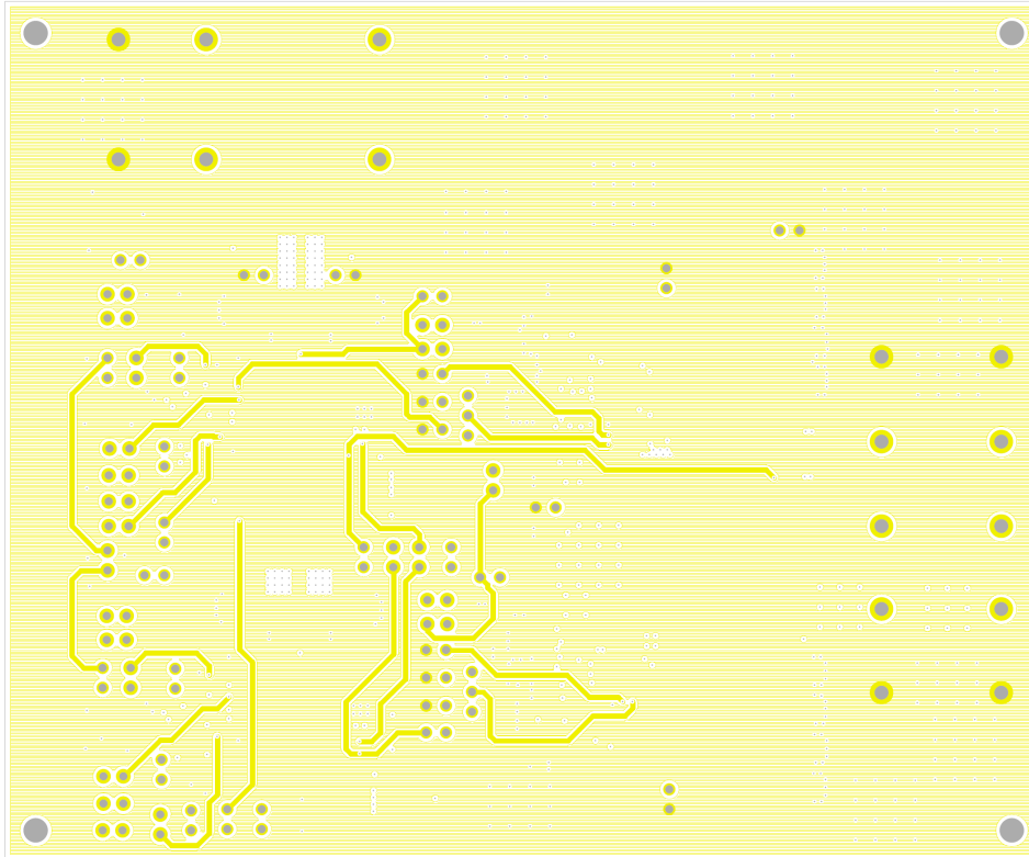
Figure 8. Layer 4
