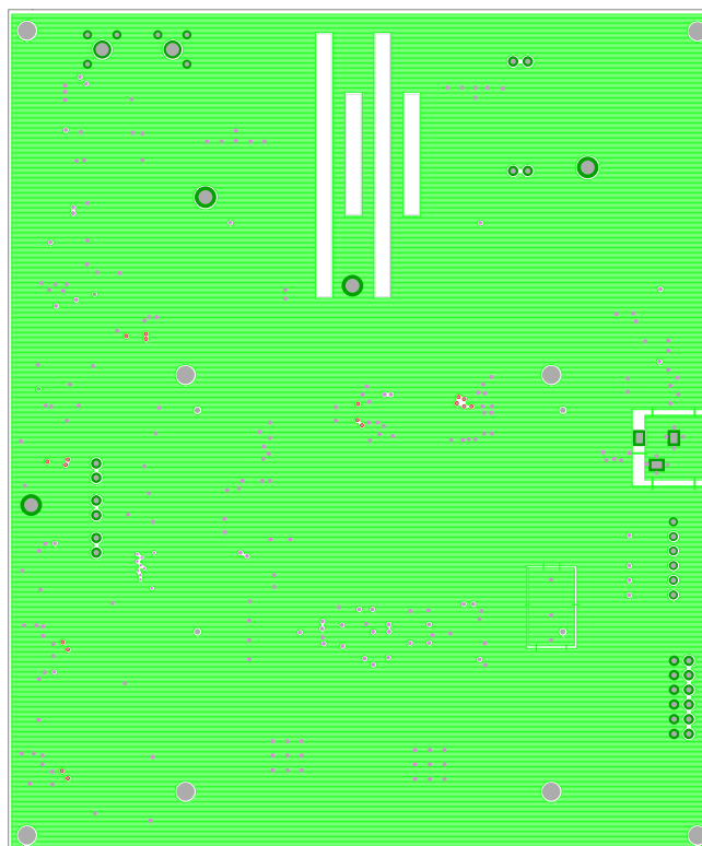
Figure 39. Layer 2
