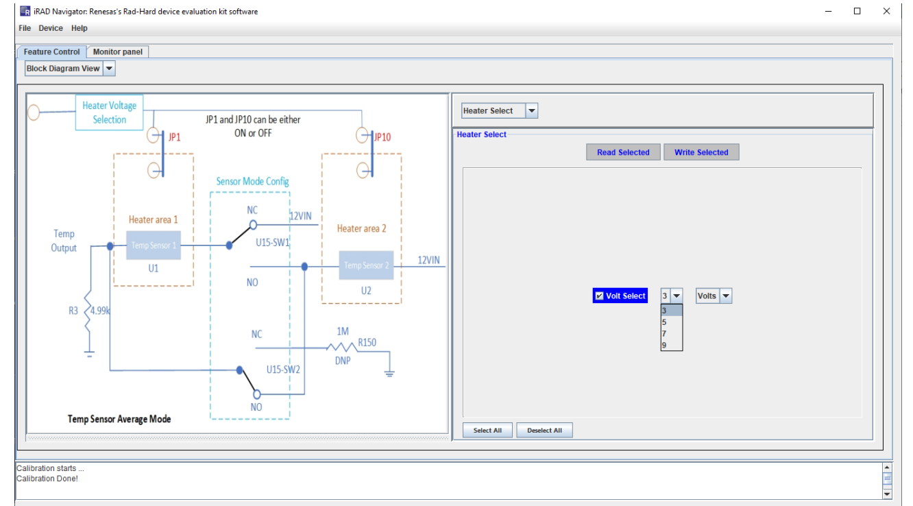
Figure 20. iRADNavigator Heater Voltage Selection
