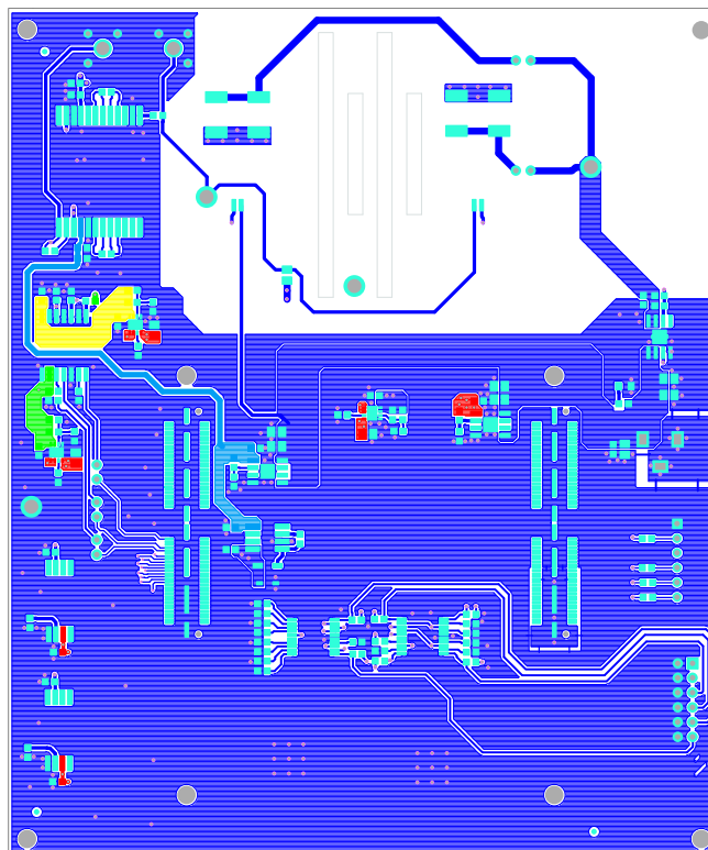
Figure 38. Top Layer
