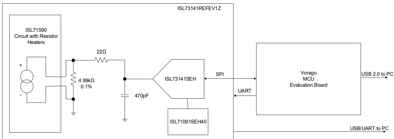
Figure 1. Block Diagram
