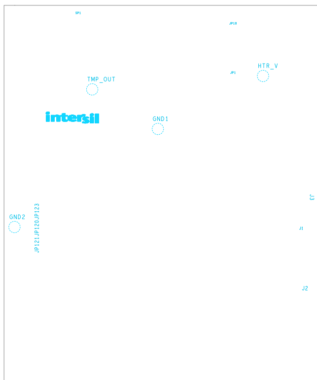
Figure 42. Bottom Silkscreen
