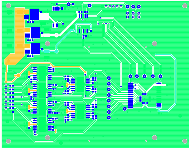
Figure 34. Top Layer
