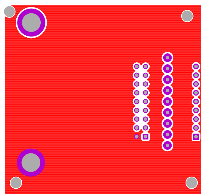
Figure 39. Bottom Layer
